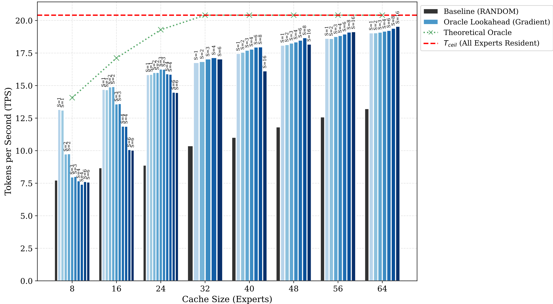
Oracle Throughput by Lookahead and Cache Size
