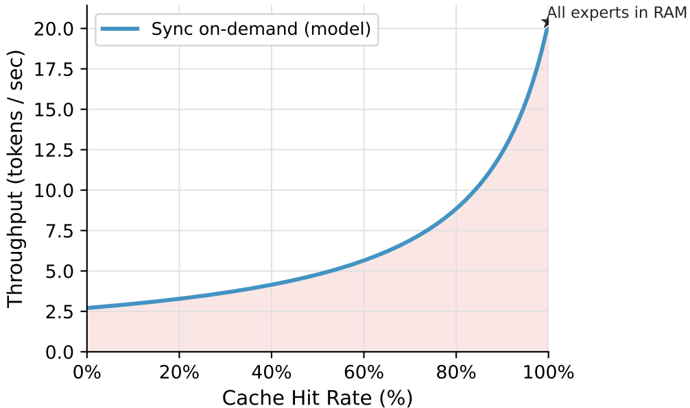
Throughput vs. Cache Hit Rate (synchronous on-demand SSD loads for misses)
