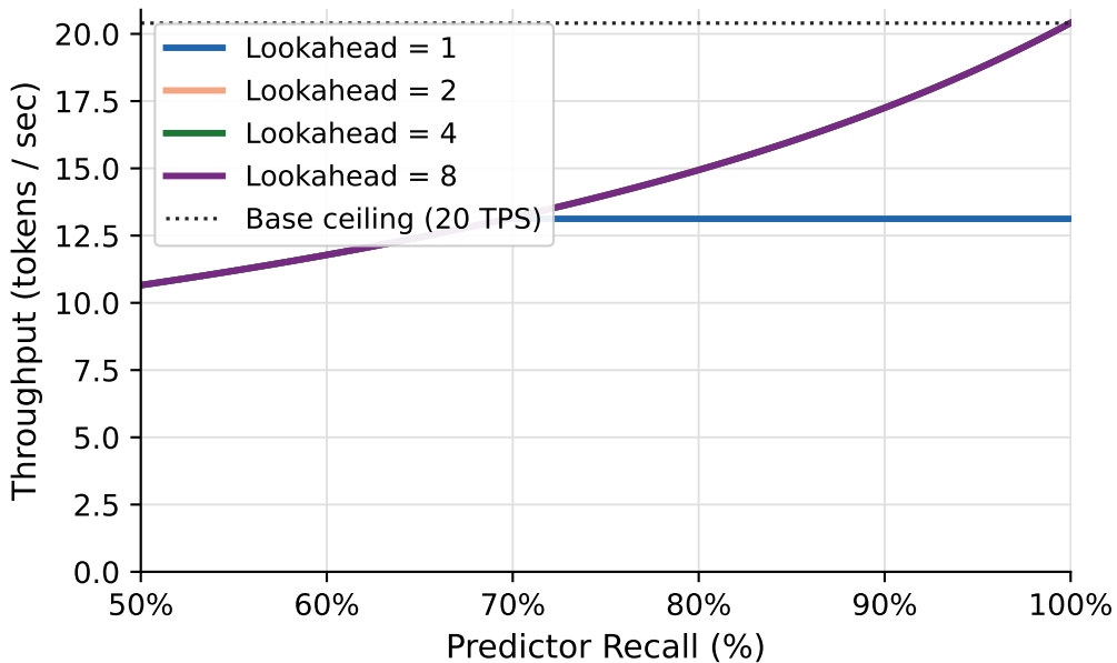
Throughput vs. Predictor Recall (by lookahead depth, fixed precision \approx 85\% )
