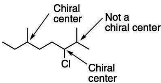
Figure 65: Chiral and non-chiral center examples
