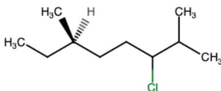
Figure 67: Left methyl substituent from Figure 65 as a wedge
