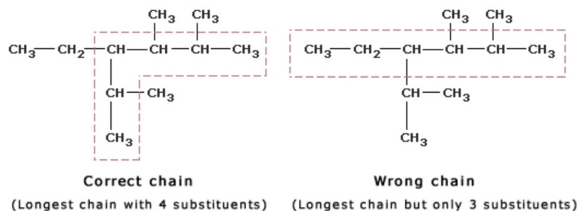
Figure 40: Identifying the parent chain
