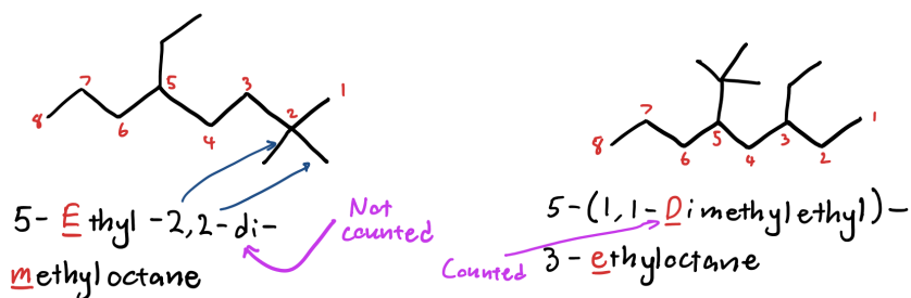
Figure 51: Alphabetical counting of prefixes; EXPLANATION PLACEHOLDER
