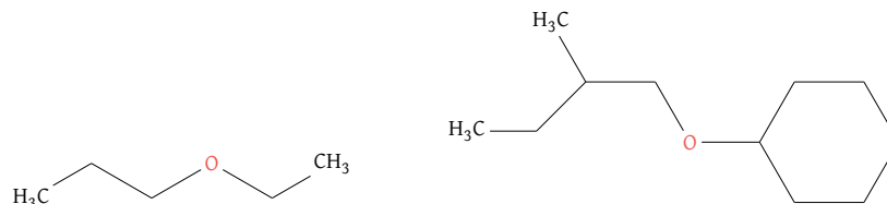
Figure 61: Ether nomenclature examples
