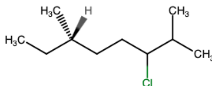
Figure 69: Left methyl substituent from Figure 65 as a dash
