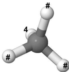
Figure 66: Absolute configuration perspective visualized
