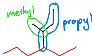
Figure 42: Methylpropyl branched substituent
