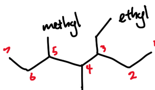
Figure 48: Alphabetical numbering of parent chain when substituent position is mirrored; ethyl precedes methyl alphabetically, therefore numbering commences from the right terminus
