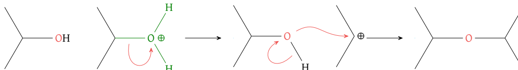
Figure 8: Symmetrical ether formation via S_N1
