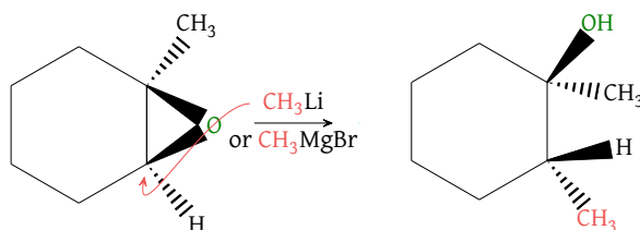
Figure 15: Stereocontrolled ether ring opening
