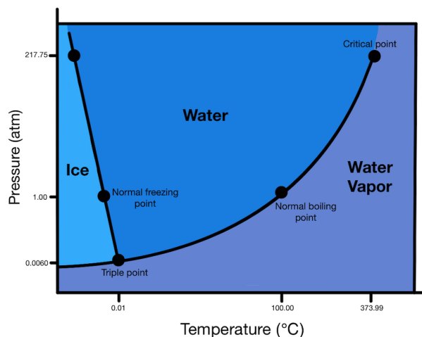
Figure 6: Phase diagram of water
