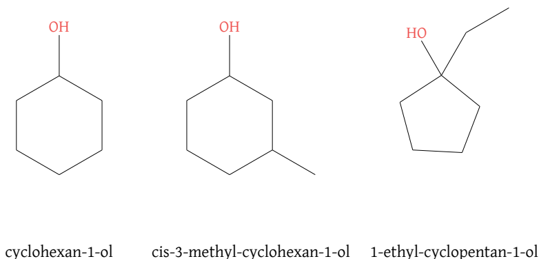
Figure 56: Cycloalkanol nomenclature examples
