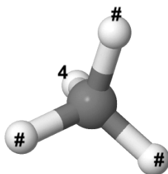
Figure 63: Absolute configuration perspective visualized
