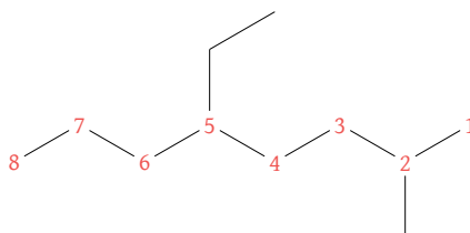
5- E thyl-2- m ethyloctane
