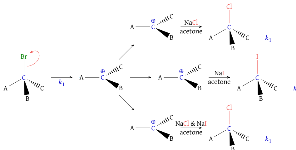
Figure 19: S_N1 nucleophile competition; \text{Cl}^- is a better nucleophile than \text{I}^- , thus a mixture will result in the \text{Cl}^- product (bottom reaction)
