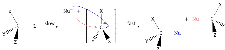
Figure 17: S_N1 mechanism
