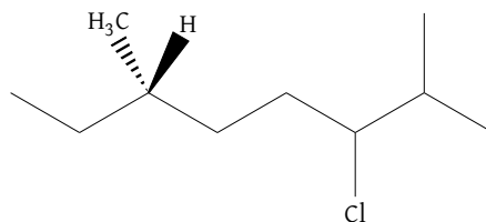
Figure 66: Left methyl substituent from Figure 62 as a dash
