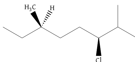
Figure 67: (3S,6R)-3-chloro-2,6-dimethyloctane
