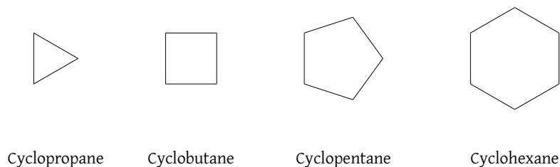
Figure 51: Cycloalkanes
