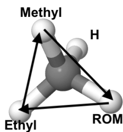
Figure 65: R configuration
