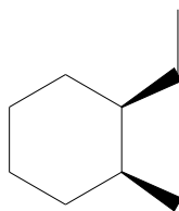
Figure 68: (1R,2S)-1-ethyl-2-methylcyclohexane
