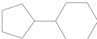
Figure 54: Cyclopentylcyclohexane
