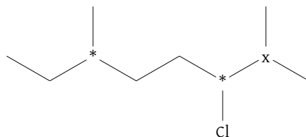
Figure 62: Chiral (*) and non-chiral (x) center examples
