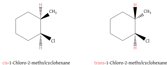
Figure 61: Cis and trans isomers
