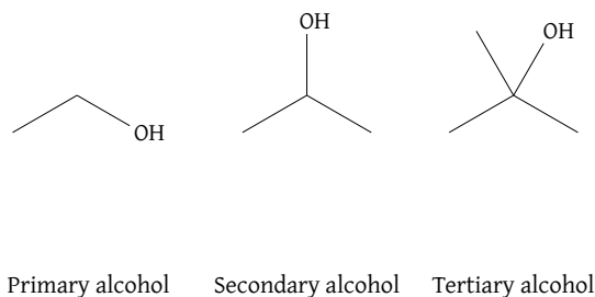
Figure 57: Primary, secondary, and tertiary alcohols
