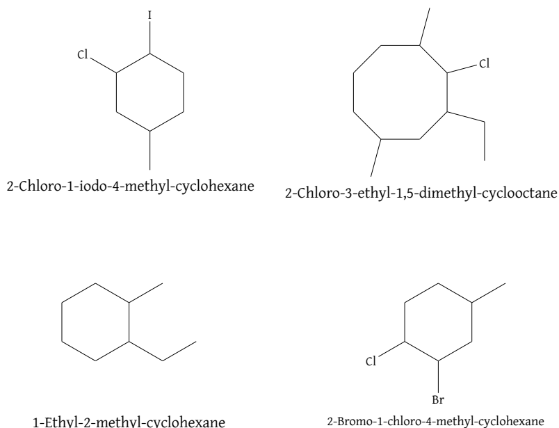
Figure 53: Cycloalkane nomenclature examples
