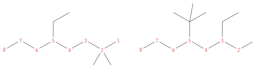
5- E thyl-2,2- d imethyloctane
