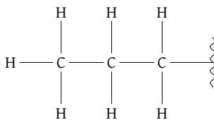
Figure 39: Propyl substituent
