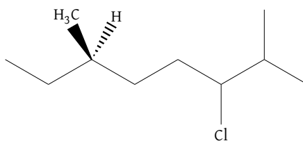
Figure 64: Left methyl substituent from Figure 62 as a wedge
