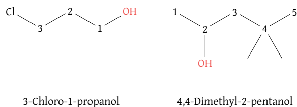
Figure 55: Alcohol nomenclature examples
