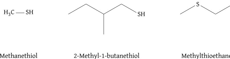
Figure 59: Thiol nomenclature examples
