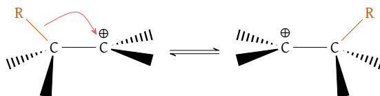
Figure 22: Alkyl shift mechanism
