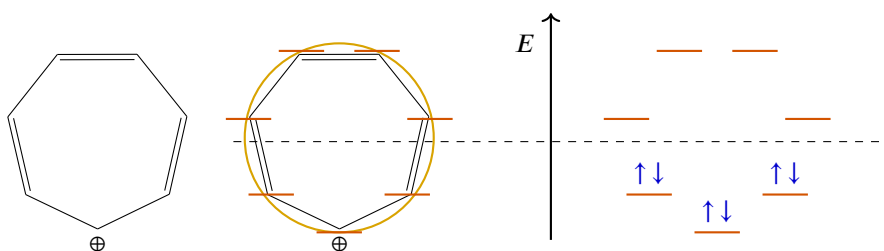
Figure 62: Frost diagram for the cycloheptenyl cation, showing three filled bonding/nonbonding orbitals and four unoccupied, degenerate antibonding orbitals
