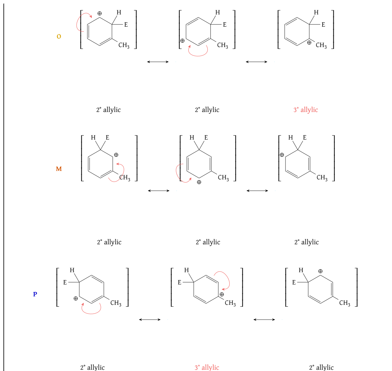
Figure 90: Ortho, meta, para positioning resonance structures of \text{H}_3\text{CPh}
