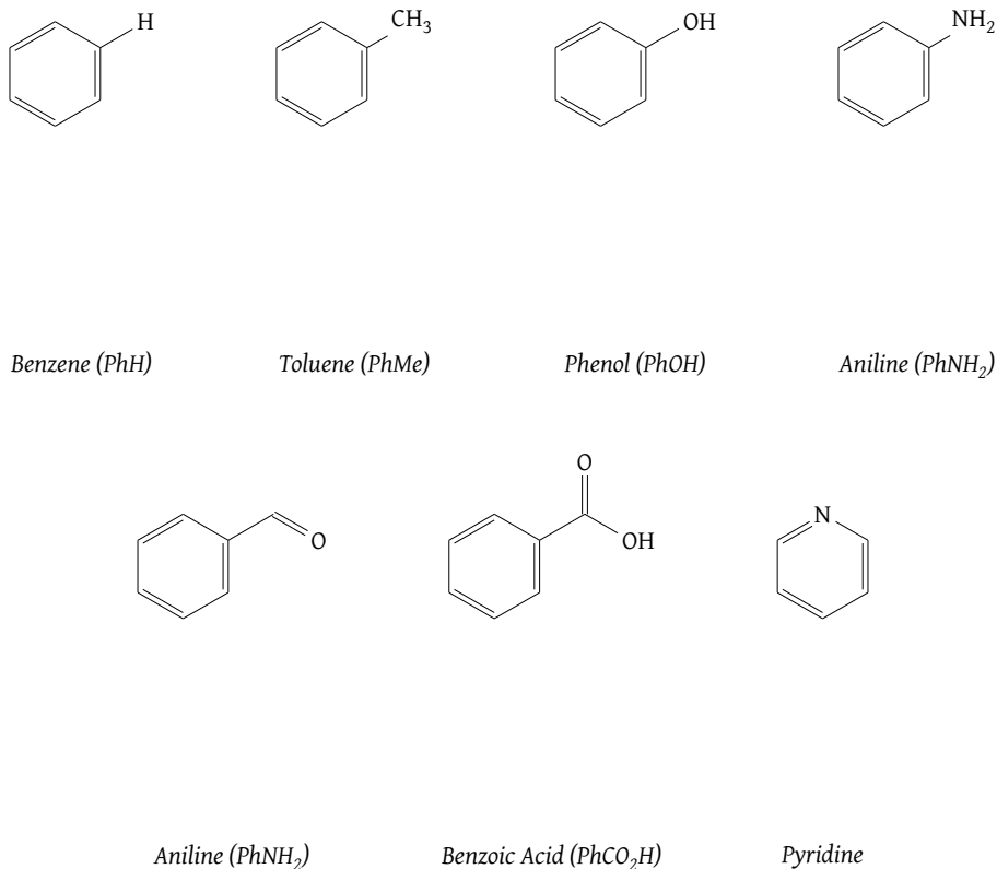
Figure 55: Phenyl ring-based aromatic compound examples; pyridine represents an aromatic compound with a non-CH atom as part of its ring
