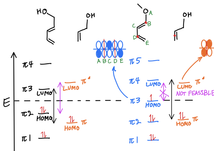
Figure 52: Diels–Alder reaction electronic effects; the reagents on the left actually react faster despite the smaller \pi_3 – \pi_4^* gap of the reagents on the right, because the latter possesses a node on the atom required to form a new \sigma bond
