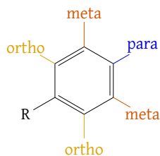
Figure 56: Phenyl ring substituent-positioning keywords
