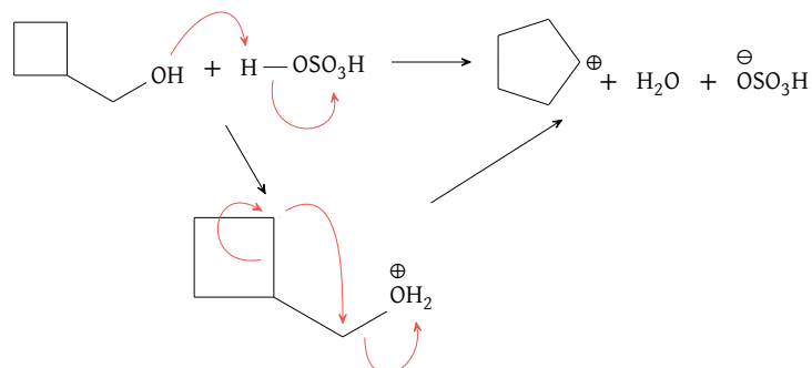
Figure 82: Acid-catalyzed dehydration and subsequent ring expansion to generate a more thermodynamically stable cyclopentyl carbocation
