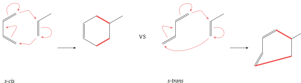
Figure 49: s-cis (left) versus s-trans (right) diene orientation; the s-trans orientation induces substantial ring strain; a ring must contain at least eight atoms to accommodate a trans \pi bond, and consequently the s-trans reaction depicted above does not proceed
