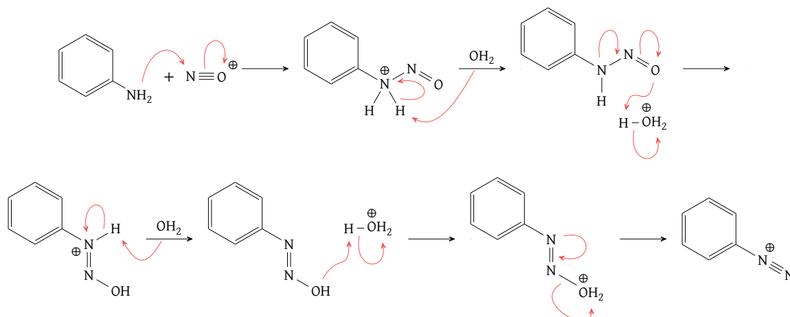
Figure 106: Conversion of aniline to aryl diazonium via interaction with the nitrosyl cation
