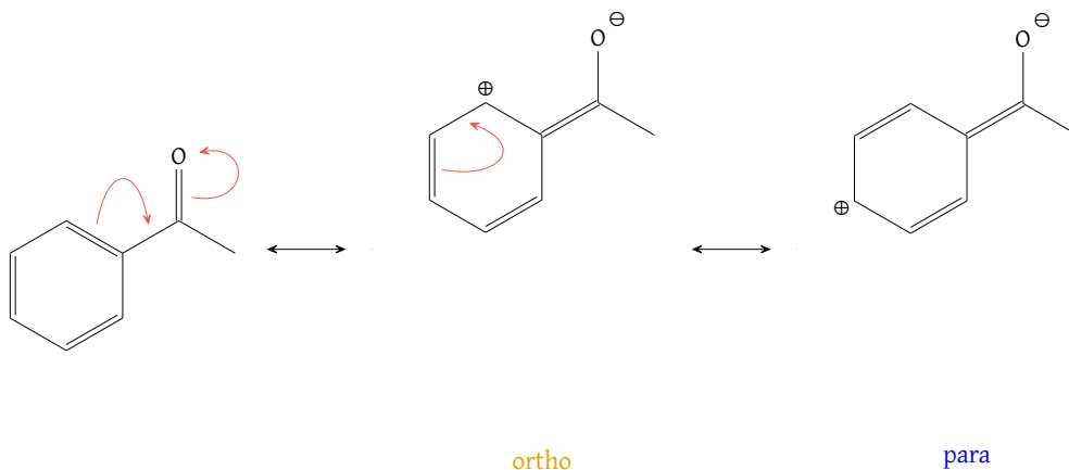
Figure 97: Resonance M director
