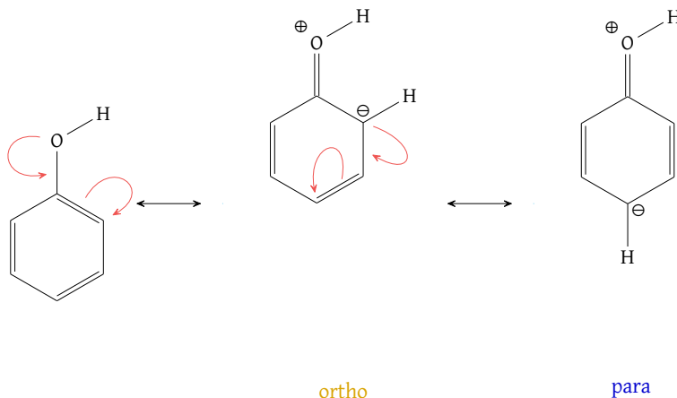
Figure 95: Resonance O/P director; this mechanism requires a substituent capable of donating an electron pair
