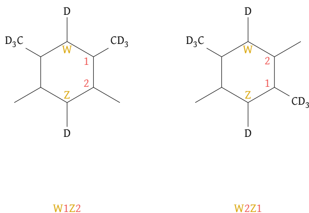
Figure 48: Isomer product possibilities of the reaction shown in Figure 47
