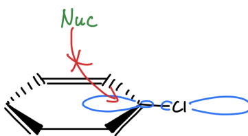
Figure 112: Backside nucleophilic attack on the carbon of chlorobenzene, prevented by steric hindrance from the aromatic ring
