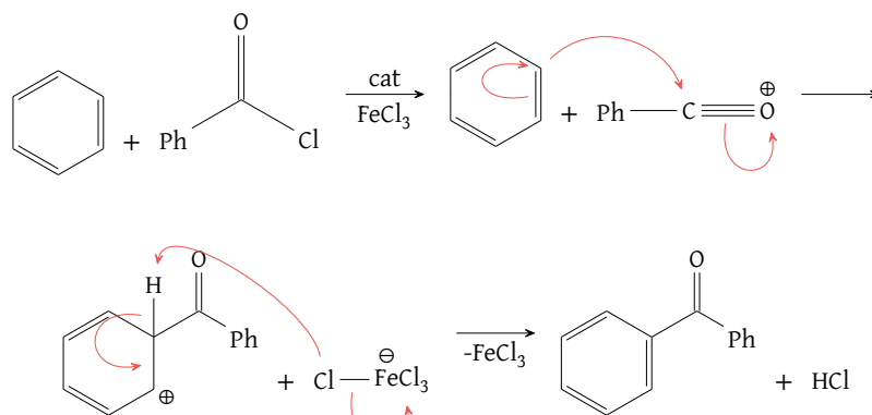
Figure 87: Acylation of benzene
