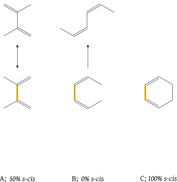
Figure 50: Differences in s-cis orientation prevalence across the three dienes; Diels-Alder reaction rates favor diene C the most and diene B the least
