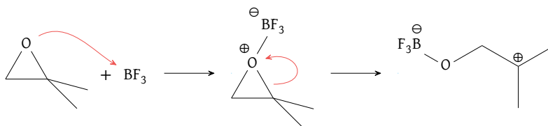
Figure 79: Boron trifluoride ( \text{BF}_3 ) coordination to an epoxide, promoting regioselective ring cleavage to generate the more thermodynamically stable tertiary carbocation
