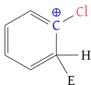
Figure 100: Inductive effect
