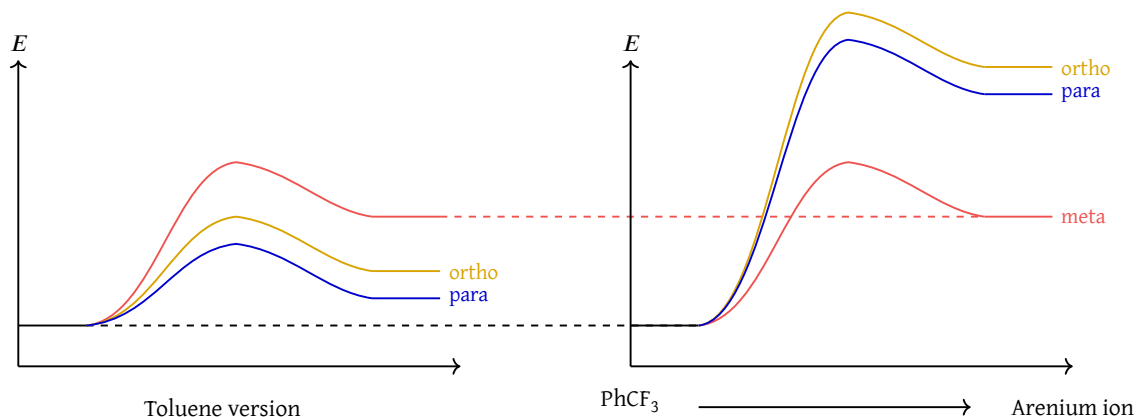
Figure 94: Energy diagram comparing the transition-state energies for meta, ortho, and para substitution in the reactions \text{H}_3\text{CPh} + \text{E}^+ \longrightarrow \text{H}_3\text{CPhE}^+ and \text{F}_3\text{CPh} + \text{E}^+ \longrightarrow \text{F}_3\text{CPhE}^+ ; inductive directors raise the O/P energies comparatively more, making meta the relatively favored position
