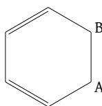
Figure 63: Nonaromatic cyclohexene; carbons A and B are sp^3 , which prevents an uninterrupted cyclic array of p orbitals
