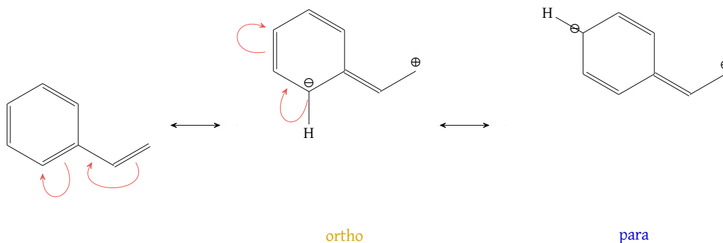
Figure 96: Conjugated \pi system resonance O/P directing
