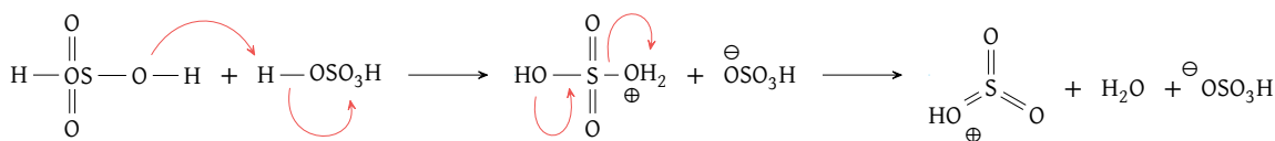
Figure 76: Formation of fuming \text{H}_2\text{SO}_4
