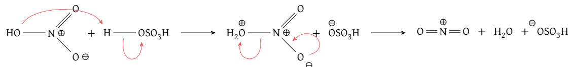
Figure 74: Generation of the \text{NO}_2^+ electrophile
