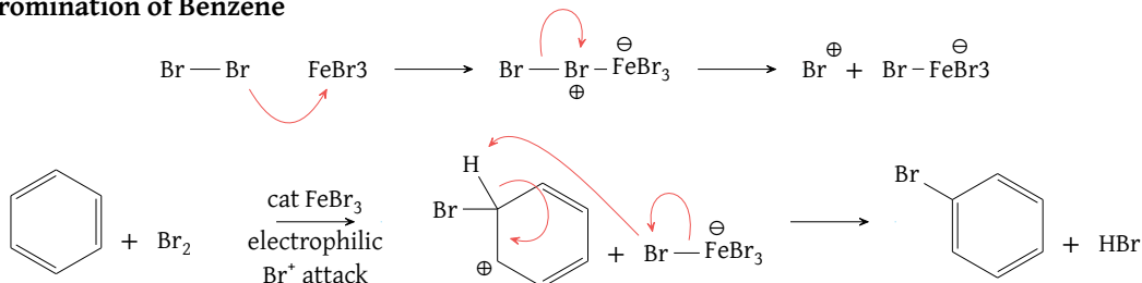
Figure 73: Bromination of benzene
