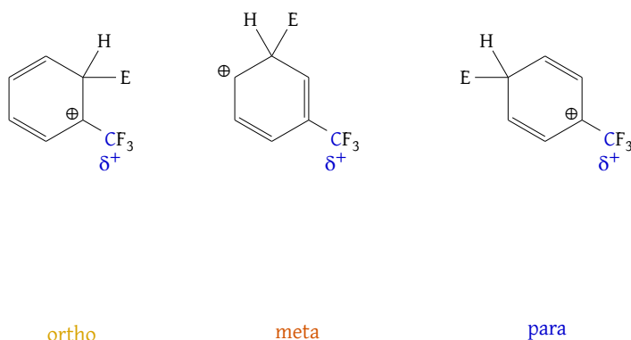
Figure 93: Best resonance contributors of each position in \text{F}_3\text{CPh} ; the O/P 3° allylic contributors experience additional Coulombic repulsion due to the partially positive adjacent carbon of the \text{CF}_3 substituent
