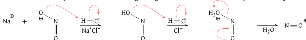
Figure 105: Conversion of \text{NO}_2^- to a nitrosyl cation
