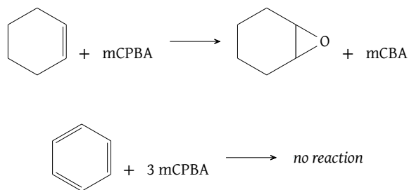
Figure 58: Reactions of cyclohexene and benzene with mCPBA
