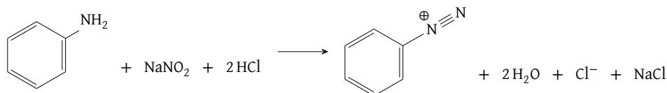
Figure 104: Diazotization of aniline
