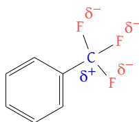
Figure 92: Inductive M directors
