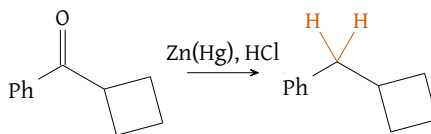
Figure 85: Reduction of ketone with Zn(Hg) and HCl
