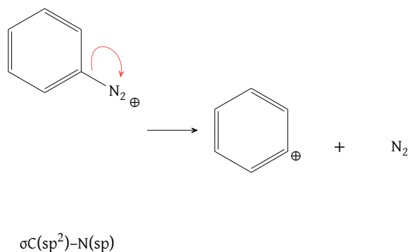
Figure 107: Diazonium chemistry; note that the empty orbital is the \text{sp}^2 orbital rather than the p orbital, meaning no resonance is available to stabilize the resulting positive charge
