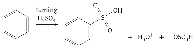
Figure 77: Sulfonation of benzene
