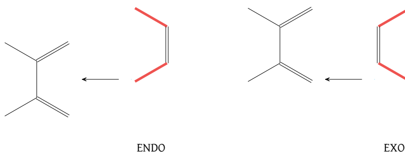
Figure 44: Endo (left) and exo (right) attack by the dienophile in a Diels–Alder reaction
