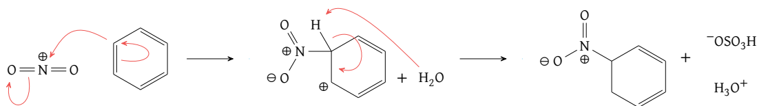
Figure 75: Nitration of benzene
