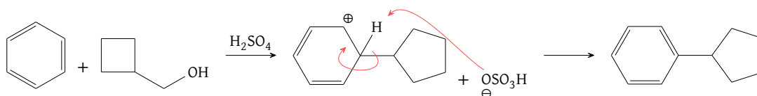
Figure 83: Electrophilic aromatic substitution of benzene by a rearranged cyclopentyl carbocation
