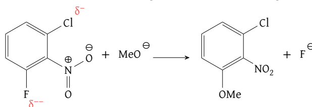
Figure 115: NAS addition/elimination practice example 1 — the correct reaction pathway
