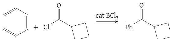
Figure 84: Acylation
