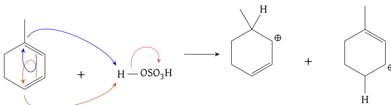
Figure 81: Electrophilic attack on toluene by \text{H}^+ ; the first hydrogenation step follows either the blue or orange e^- movement
