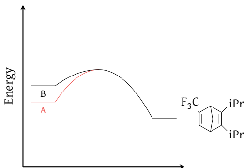
Figure 54: Energy diagrams for the corresponding diene-dienophile pairs from Figure 53; the E_a for compound pair B is substantially smaller than that of pair A, owing to the former's relatively higher starting energy state
