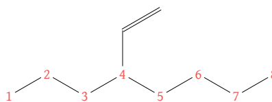
4-vinyl-octane
