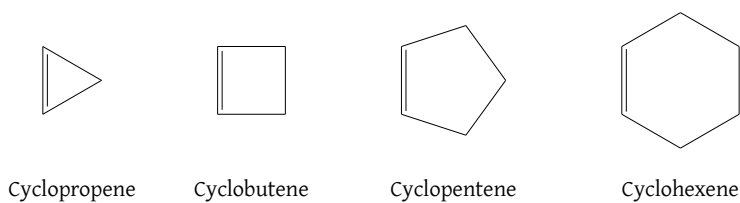
Figure 60: Cycloalkenes
