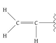
Vinyl ( Ethenyl )
