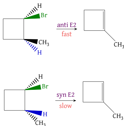
Figure 26: Anti and syn-periplanar E2 reaction rates
