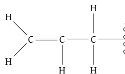
Allyl ( Prop-2-enyl )
