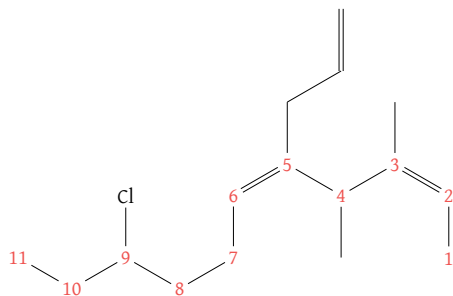
Figure 59: (2Z,5Z)-5-Allyl-9-chloro-3,4-dimethyl-undec-2,5-diene
