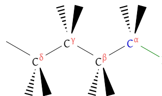
Figure 16: Carbon branching
