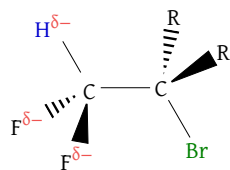
Figure 24: E2 hydrogen acidity amplification
