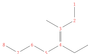
4-Ethyl-3-methyl-oct-3-ene
