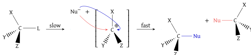
Figure 17: S_N1 mechanism
