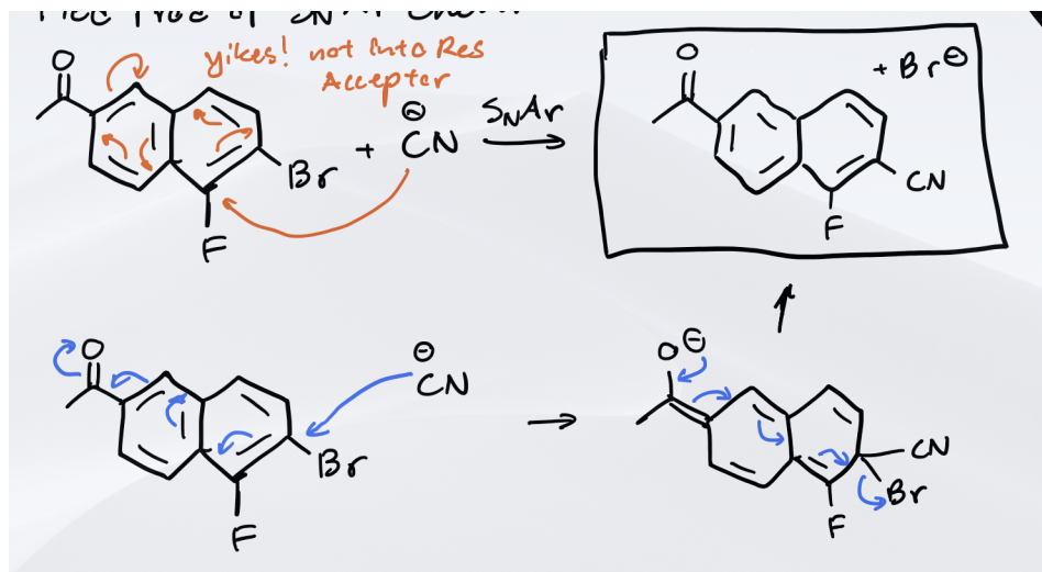
Figure 106: showcase the pathways and how one isn't possible
