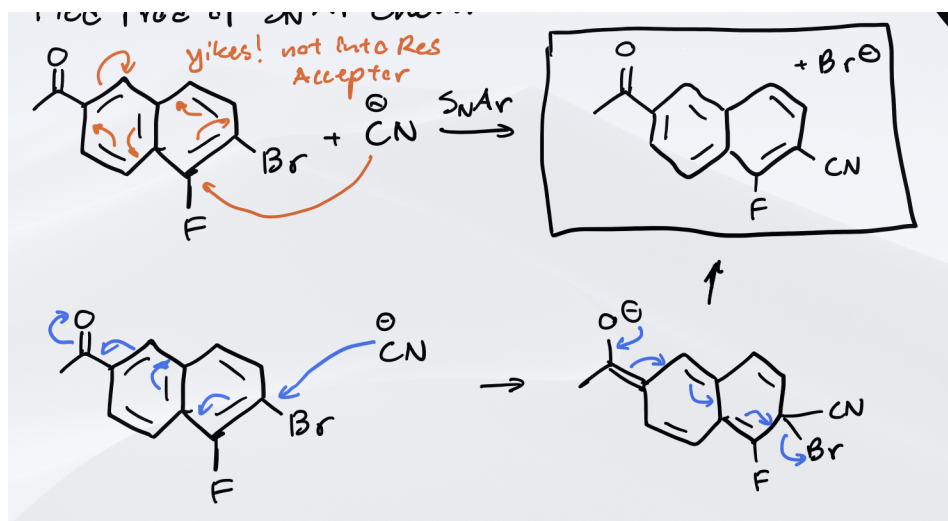
Figure 108: complete chemical equation
