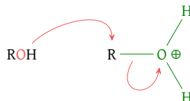
Figure 7: Symmetrical ether formation via S_N2
