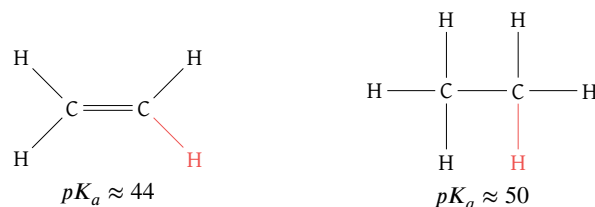
Figure 3: Ethene (left) vs ethane (right) pK_a values
