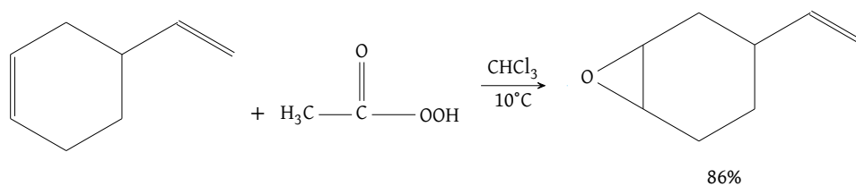
Figure 50: Rate of oxacyclopropanation increases with alkyl substitution, since hyperconjugation allows for greater e^- donation; notice that the more favorable product derives from the oxacyclopropanation of the more substituted alkene double bond
