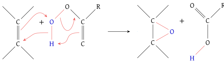
Figure 49: Mechanism of peroxycarboxylic acid addition to alkenes
