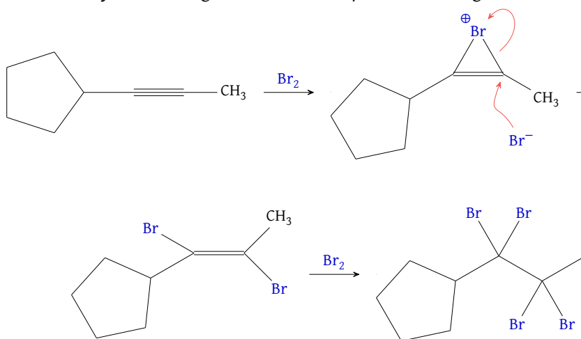
Figure 88: Anti Br 2 addition to an alkyne
