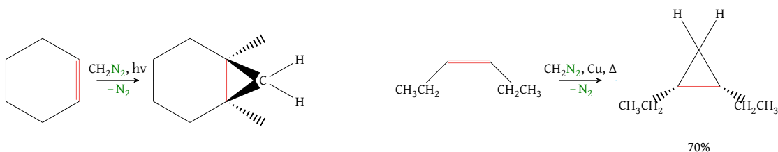
Figure 45: Examples of methylene formation from diazomethane occurring simultaneously with its addition to an alkene
