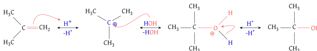
Figure 25: Markovnikov hydration mechanism; \text{H}^+ is consumed and regenerated at the start and end of the reaction process
