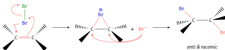
Figure 29: Halogenation (bromination) of alkenes mechanism
