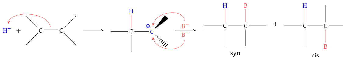
Figure 22: Outline reaction of alkene electrophilic addition; mind that the syn and cis versions have two possible arrangement as shown by the absence of dashed and wedged bonds
