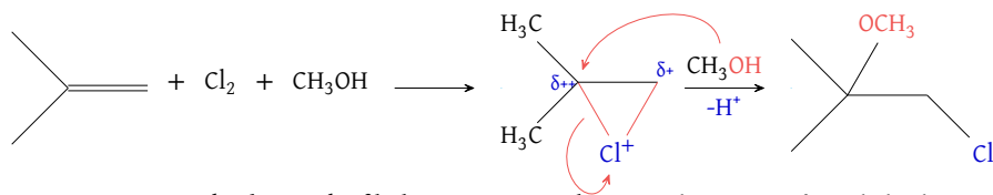
Figure 31: Backside attack of halonium ring ion by ROH; this reaction forms haloethers
