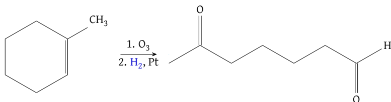
Figure 59: Ozonolysis reduction through catalytic hydrogenation; this reaction yields a cycloalkene ring opening
