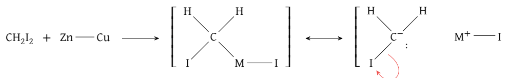
Figure 42: Simmons-Smith reagent methylene formation
