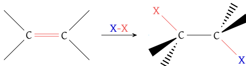
Figure 28: Outline alkene halogenation reaction; notice that X_2 gets polarized during approach to alkene
