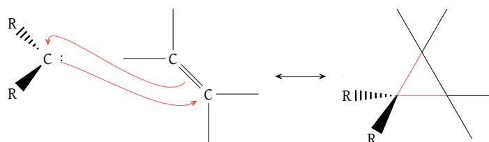
Figure 43: Outline reaction of electrophilic carbene additions to alkenes
