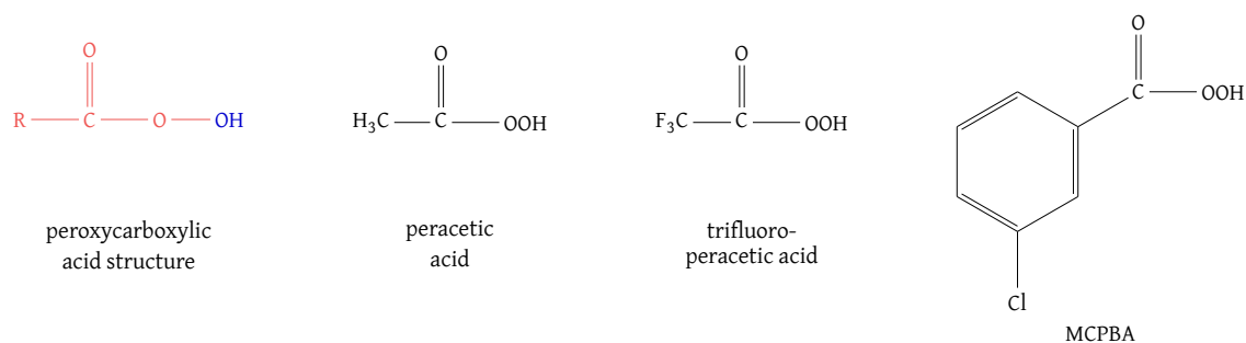
Figure 47: General peroxycarboxylic acid structure (left) and commonly used peroxycarboxylic acids
