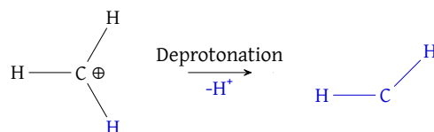
Figure 39: Deprotonation of carbocation
