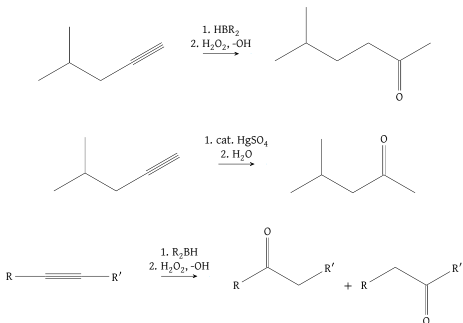
Figure 95: Hydroboration-oxidation (top, bottom) vs mercury catalyzed Markovnikov hydration (middle)
