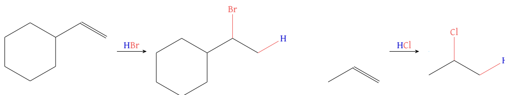
Figure 23: Hydrobromination (left) and hydrochlorination (right)
