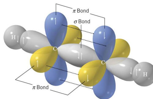
Figure 64: Alkyne triple bond orbital structure
