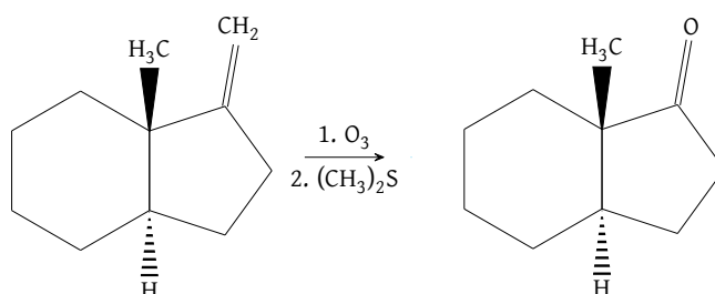
Figure 60: Ozonolysis reduction through dimethyl sulfide (DMS); this reaction yields a "clipped off" carbon atom
