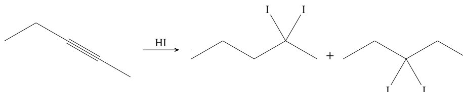
Figure 84: Asymmetrical internal alkyne HX anti addition
