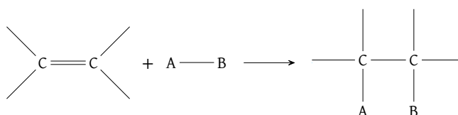
Figure 18: Outline alkene addition reaction; this reaction is usually exothermic
