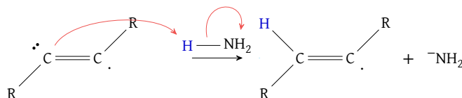
Figure 79: Sodium reduction first protonation
