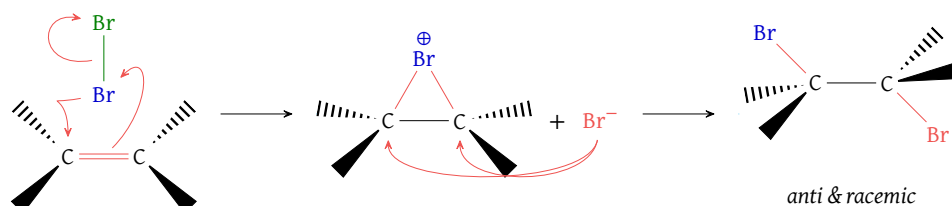
Figure 29: Halogenation (bromination) of alkenes mechanism
