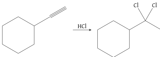
Figure 85: Terminal alkyne HX anti addition
