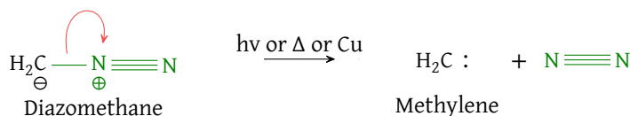
Figure 40: Methylene from diazomethane
