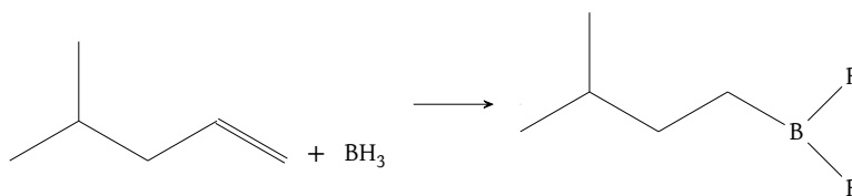
Figure 36: Hydroboration of terminal alkene; mind that the \text{R} groups in the product is the same as the one fully displayed alkyl substituent; notice that the boron attaches to the less hindered end of the terminal alkene double bond
