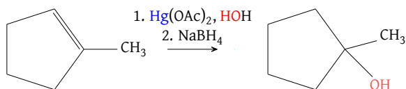
Figure 32: Oxymercuration–demercuration chemical reaction
