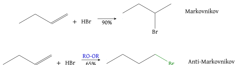
Figure 61: Markovnikov (top) vs anti-Markovnikov (bottom) \text{HBr} addition to alkene double bond; the radical anti-Markovnikov version is much faster
