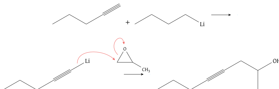
Figure 71: Terminal alkyne nucleophilicity in the presence of an oxacyclopropane
