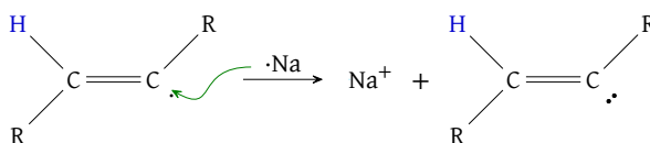
Figure 80: Sodium reduction second e^- transfer
