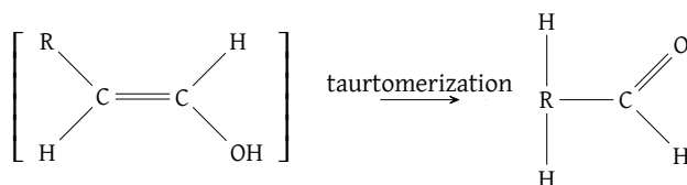
Figure 94: Tautomerization
