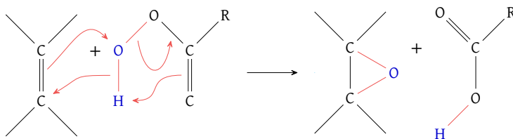
Figure 49: Mechanism of peroxycarboxylic acid addition to alkenes
