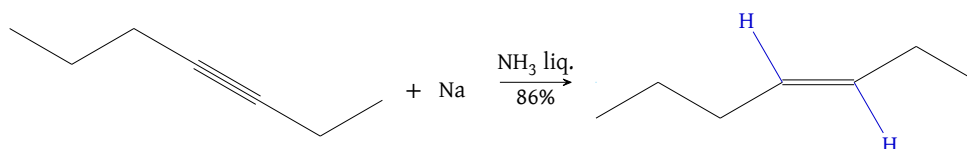
Figure 77: Partial anti hydrogenation of an alkyne with sodium reduction producing trans-3-heptene
