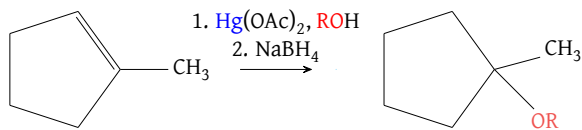
Figure 33: Oxymercuration–demercuration chemical reaction using ROH
