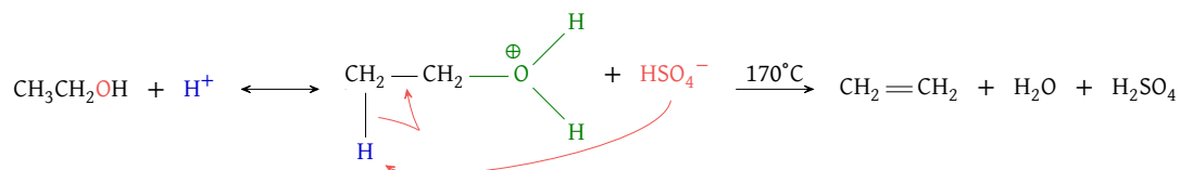
Figure 15: Alcohol dehydration example using \text{H}_2\text{SO}_4 and ethanol; \text{HSO}_4^- unusually acts as a base in this scenario
