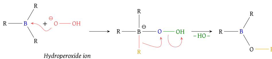
Figure 38: Oxidation of BR_3
