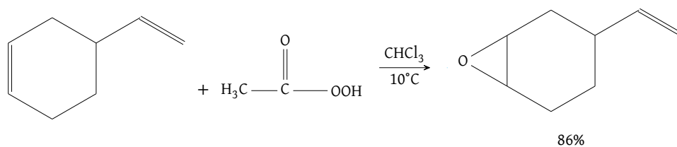
Figure 50: Rate of oxacyclopropanation increases with alkyl substitution, since hyperconjugation allows for greater e^- donation; notice that the more favorable product derives from the oxacyclopropanation of the more substituted alkene double bond
