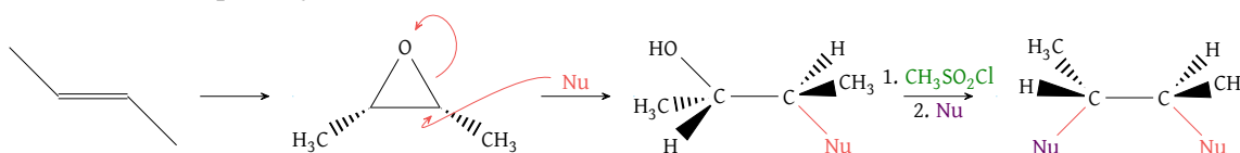
Figure 51: Double nucleophilic syn addition to alkene double bond; \text{CH}_3\text{SO}_2\text{Cl} turns the \text{OH} group into a sulfonate leaving group
