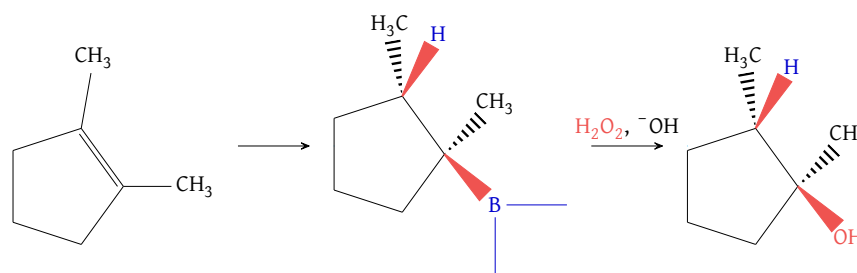
Figure 37: Syn addition of B-H
