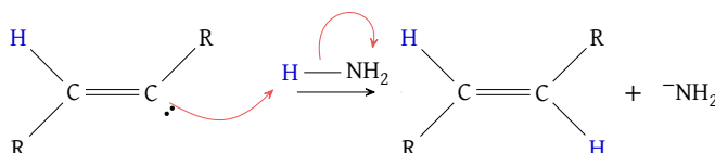
Figure 81: Sodium reduction second protonation
