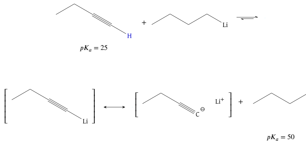
Figure 66: Alkyne acidity and organolithium reagents
