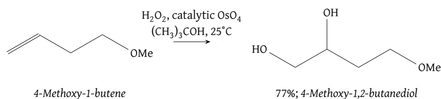
Figure 55: Catalytic \text{OsO}_4 through \text{H}_2\text{O}_2
