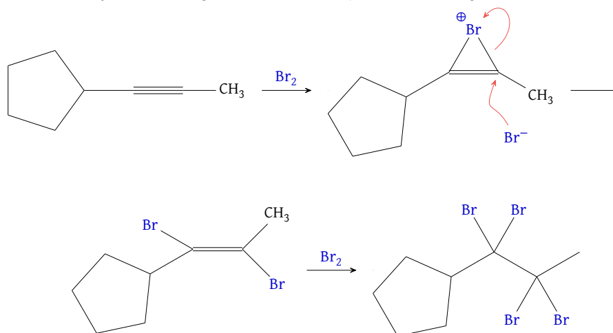
Figure 87: Anti \text{Br}_2 addition to an alkyne
