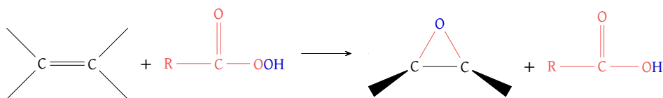
Figure 48: Peroxycarboxylic acid oxidation of an alkene
