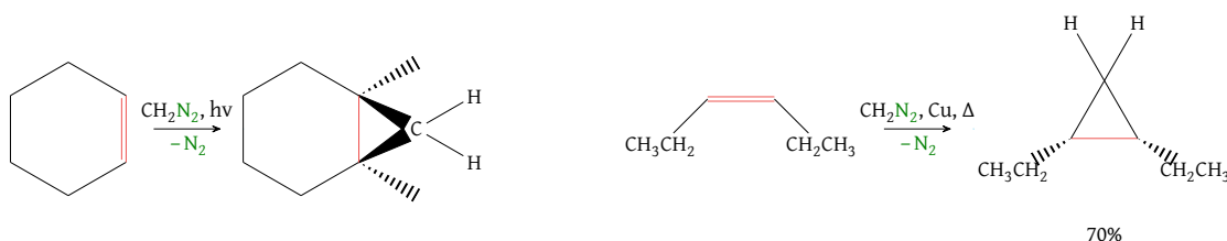
Figure 44: Examples of methylene formation from diazomethane occurring simultaneously with its addition to an alkene
