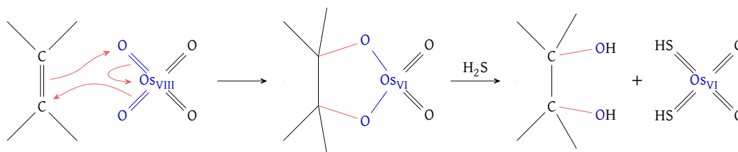
Figure 54: Mechanism of syn-dihydroxylation using \text{OsO}_4
