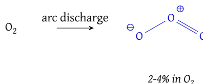
Figure 57: Laboratory formation process of ozone through arc discharge
