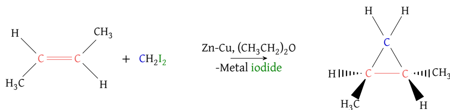
Figure 46: Simmons-Smith reagent formation occurring simultaneously with its addition to an alkene
