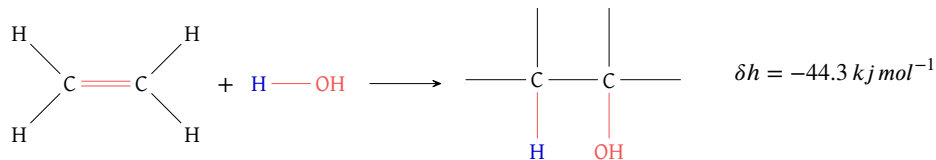
Figure 19: Alkene hydration reaction; the reaction is enthalpically favorable ( \Delta H^\circ = -44.3 \text{ kJ mol}^{-1} ) but entropically unfavorable in standard conditions, thus the Gibbs Free Energy is much lower ( \Delta G^\circ = -6.1 \text{ kJ mol}^{-1} )
