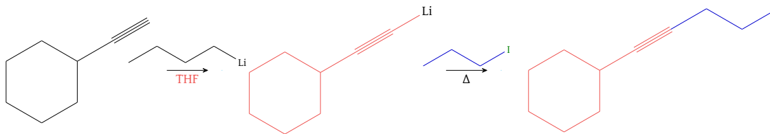
Figure 70: Strong base induced terminal alkyne nucleophilicity
