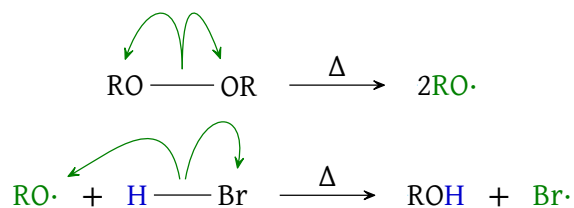
Figure 62: Initiation steps of radical hydrobromination; the formation of the radical \text{Br}\cdot begins the reaction
