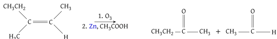
Figure 58: Ozonolysis reduction through zinc and acid
