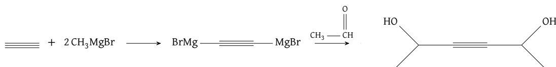
Figure 74: Double grignard addition of acetaldehyde
