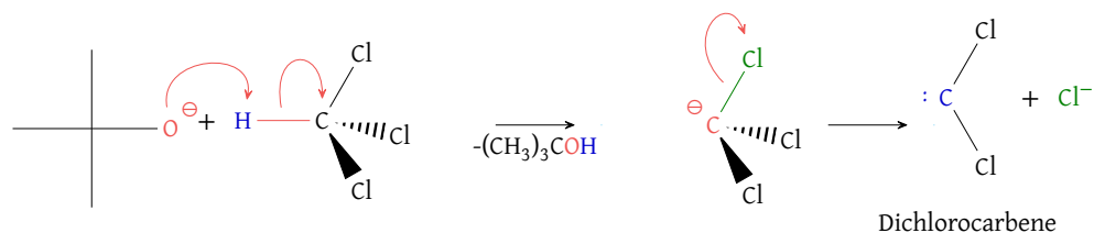
Figure 41: Dichlorocarbene from chloroform
