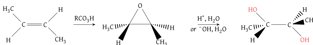
Figure 52: Anti-dihydroxylation of alkenes through oxacyclopropanation; notice that the end product is mseo , meaning it has two or more chiral centers
