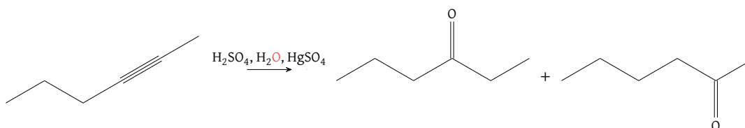
Figure 90: Mercury catalyzed Markovnikov hydration on an asymmetrical internal alkyne; both products are formed at a 50:50 ratio
