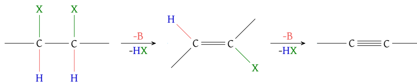
Figure 68: Synthesis of alkyne through double E2 elimination
