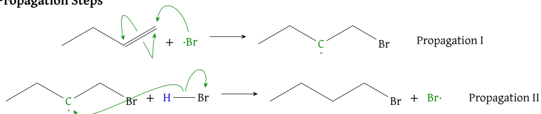
Figure 63: Propagation steps of radical hydrobromination; in regular Markovnikov, \text{H}^+ is added to the less substituted radical and then \text{Br}^- ; here, \text{Br}\cdot is added and then \text{H}\cdot ; notice that the \text{Br}\cdot is regenerated at the end to enter the next propagation cycle
