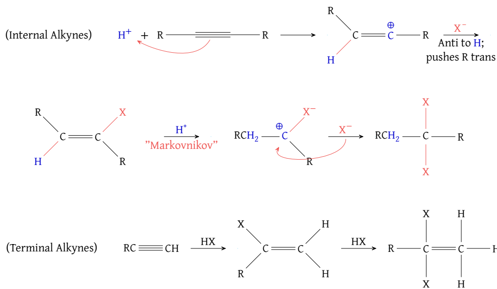
Figure 82: Double Markovnikov HX addition to alkynes resulting in geminal halides
