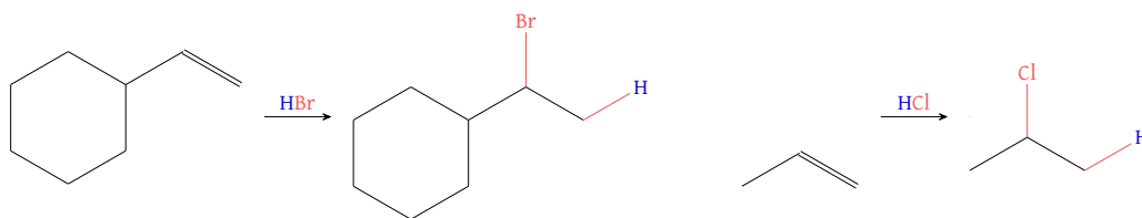
Figure 23: Hydrobromination (left) and hydrochlorination (right)
