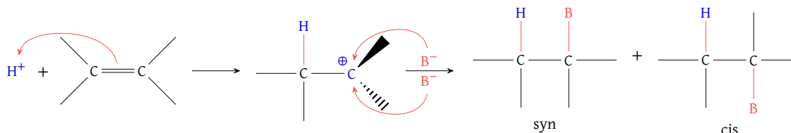
Figure 22: Outline electrophilic addition of alkene reactions; mind that the syn and cis versions have two possible arrangement as shown by the absence of dashed and wedged bonds
