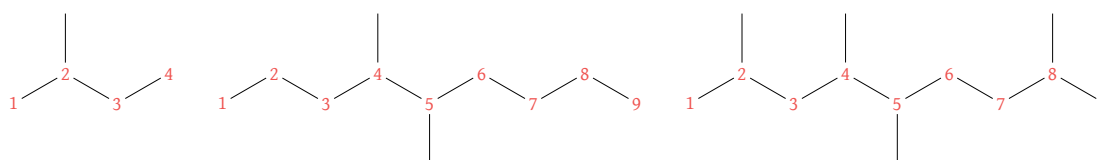
Figure 45: Numbering of parent chain in the order of earliest substituent presence (left &amp; middle) and first point of difference (right)
