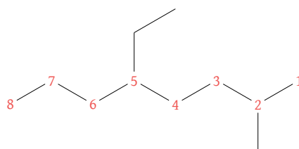
5-Ethyl-2-methyloctane
