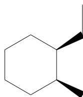
Figure 81: (1R,2S)-1-ethyl-2-methylcyclohexane
