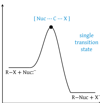
Figure 11: S_N2 energy diagram
