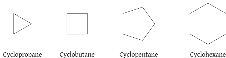
Figure 51: Cycloalkanes
