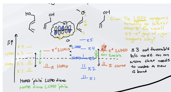
Figure 20: The left reagents actually go faster despite the small \pi_3 - \pi^* gap of the right reagents because \pi_3 is not favorable because there is a node of the atom that needs to make a new \sigma bond
