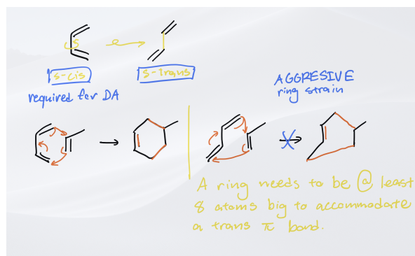
Figure 14: a ring needs to be at least 8 atoms large to accommodate a trans \pi bond
