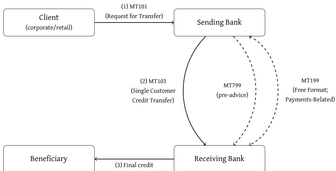
Figure 1: Overview of the MT101, MT799, MT103, and MT199 message flow in an active liquid transfer
