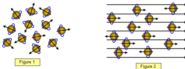
Figure 52: Proton nuclear magnetic resonance basics
