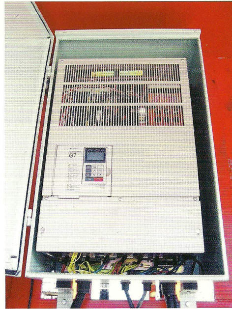
Frequency Invertor
