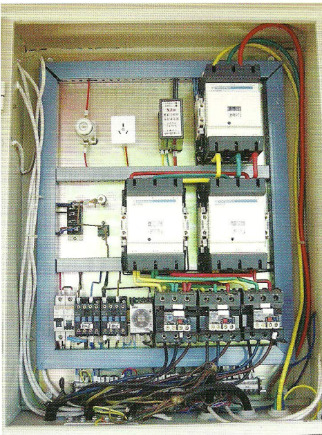
El. Cabinet
