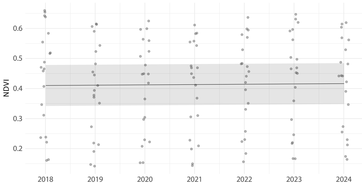
Figure 16: NDVI change over time. Mean NDVI per plot per year, based on in situ measurements from 2018 to 2024. The trend line shows a significant increase of 0.001 NDVI units per year (95% CI: 3e-04–0.0018), representing a cumulative increase of 0.0061 NDVI units over the study period.
