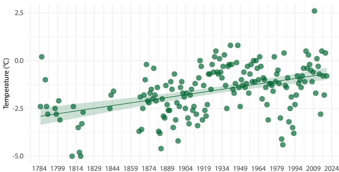
Figure 7: Historic yearly mean air temperature ( ^{\circ}\text{C} ) in Nuuk, from 1785 to 2020. Yearly mean of -1.6^{\circ}\text{C} . Yearly mean ranges from -5^{\circ}\text{C} to 2.6^{\circ}\text{C} . Modelled mean temperature has increase from -2.92^{\circ}\text{C} in 1784 to -0.65^{\circ}\text{C} in 2024 (increase of 2.27^{\circ}\text{C} or 0.095^{\circ}\text{C}/\text{decade} .)
