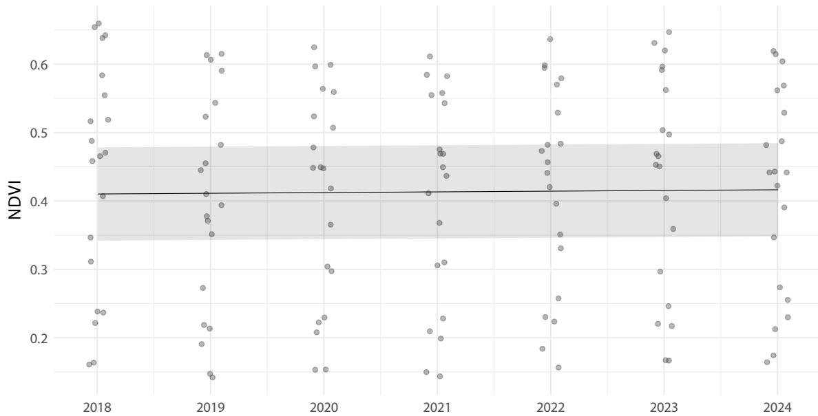
Figure 17: NDVI change over time. Mean NDVI per plot per year, based on in situ measurements from 2018 to 2024. The trend line shows a significant increase of 0.001 NDVI units per year (95% CI: 3\text{e-}04 –0.0018), representing a cumulative increase of 0.0061 NDVI units over the study period.
