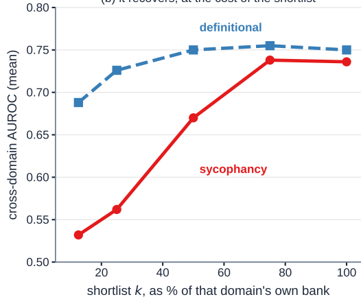
(b) it recovers, at the cost of the shortlist
