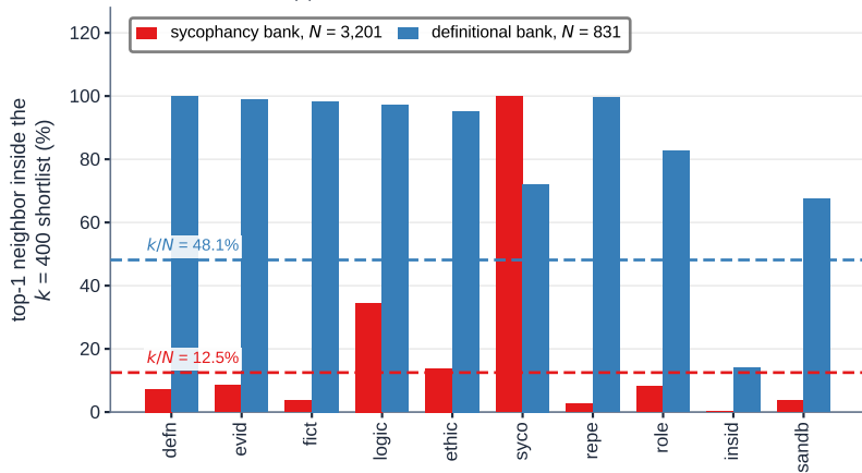
(a) a fixed k does not travel across bank sizes
