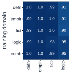
(a) published baseline (Truthfulness Spectrum, 4-domain)
