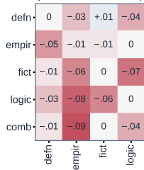
(c) fidelity change, (b) - (a) (red = AUROC lost)
