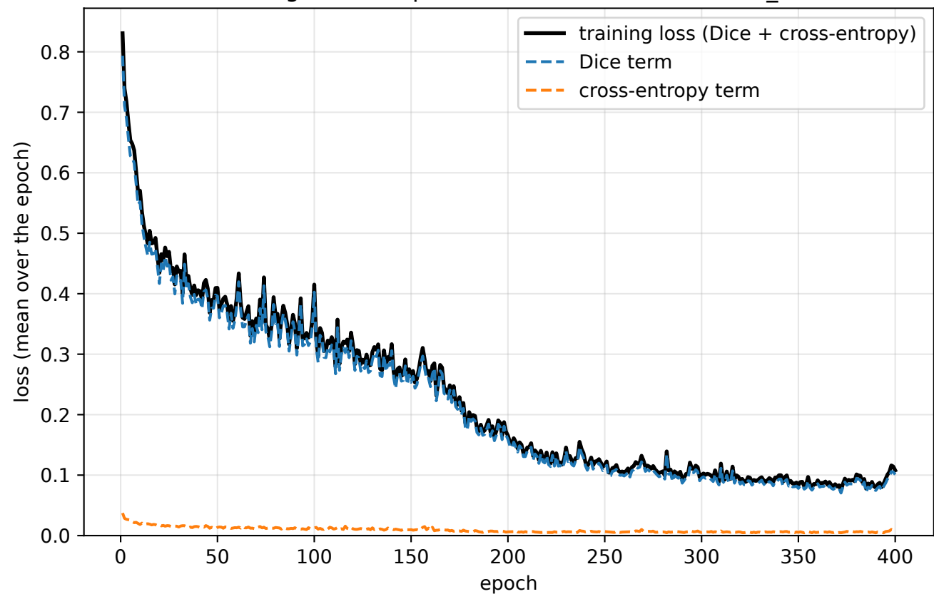
Training loss vs. epoch (raw channel 0, mask BW_I2)
