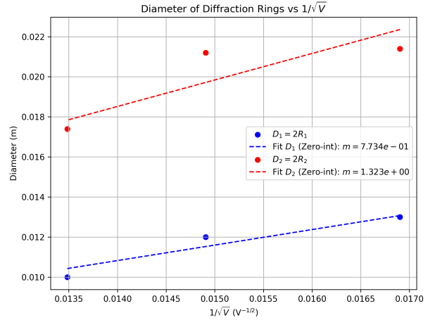
Fig. 1: Diameter of the inner ( D_1 ) and outer ( D_2 ) diffraction rings as a function of 1/\sqrt{V_a} . Dashed lines represent zero-intercept linear regressions.
