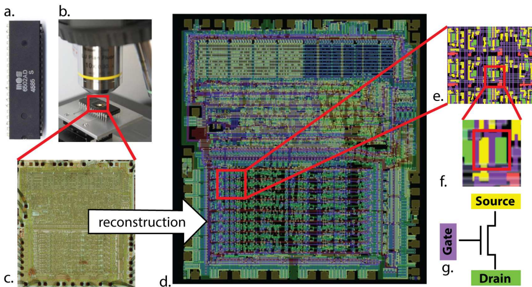
Fig 2. Optical reconstruction of the microprocessor to obtain its connectome. In [11], the (A) MOS 6502 silicon die was examined under a visible light microscope (B) to build up an image mosaic (C) of the chip surface. Computer vision algorithms were used to identify metal and silicon regions (E) to detect transistors (F), (G) ultimately producing a complete accurate netlist of the processor (D).
