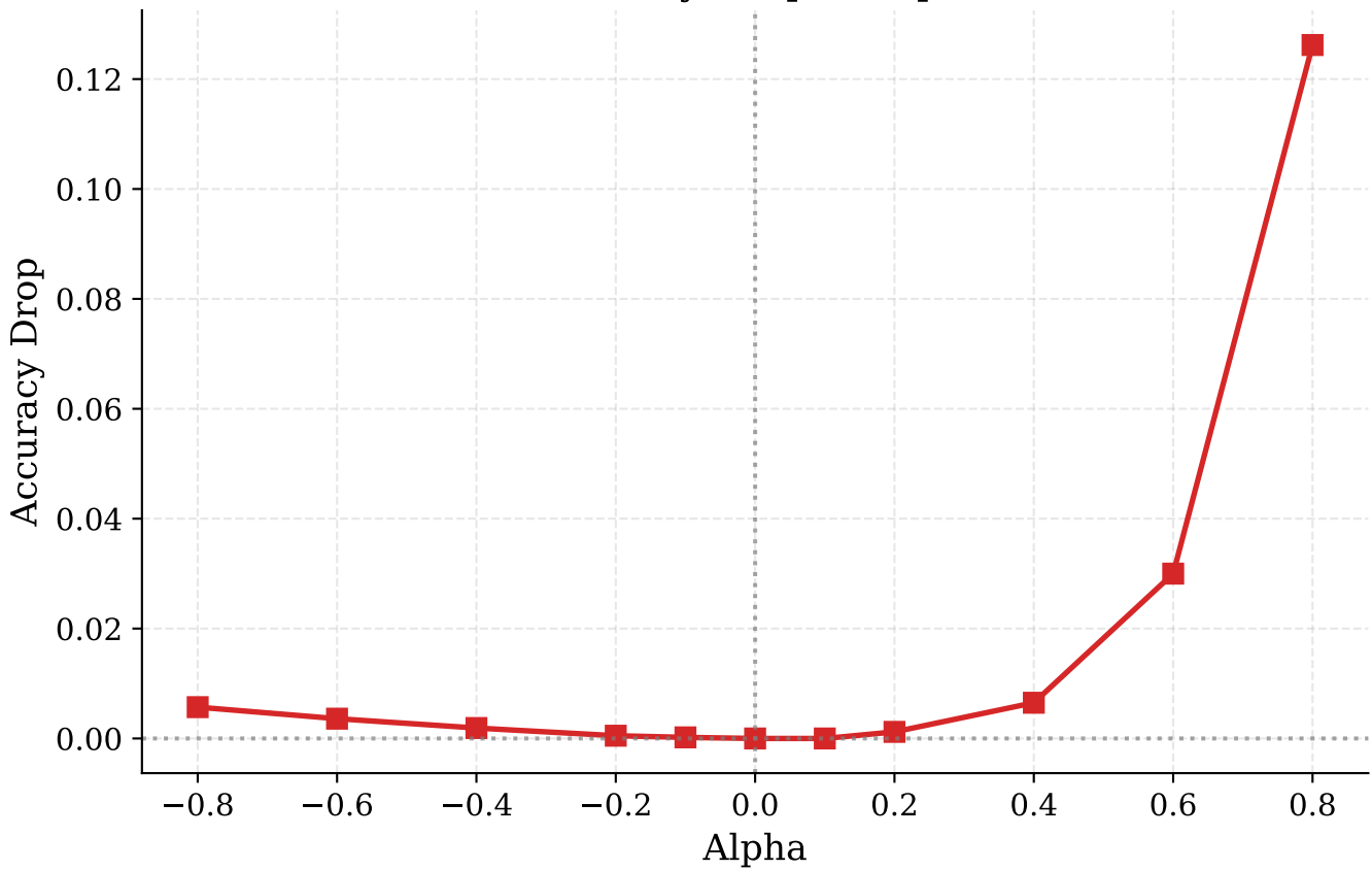
Accuracy Drop vs Alpha
