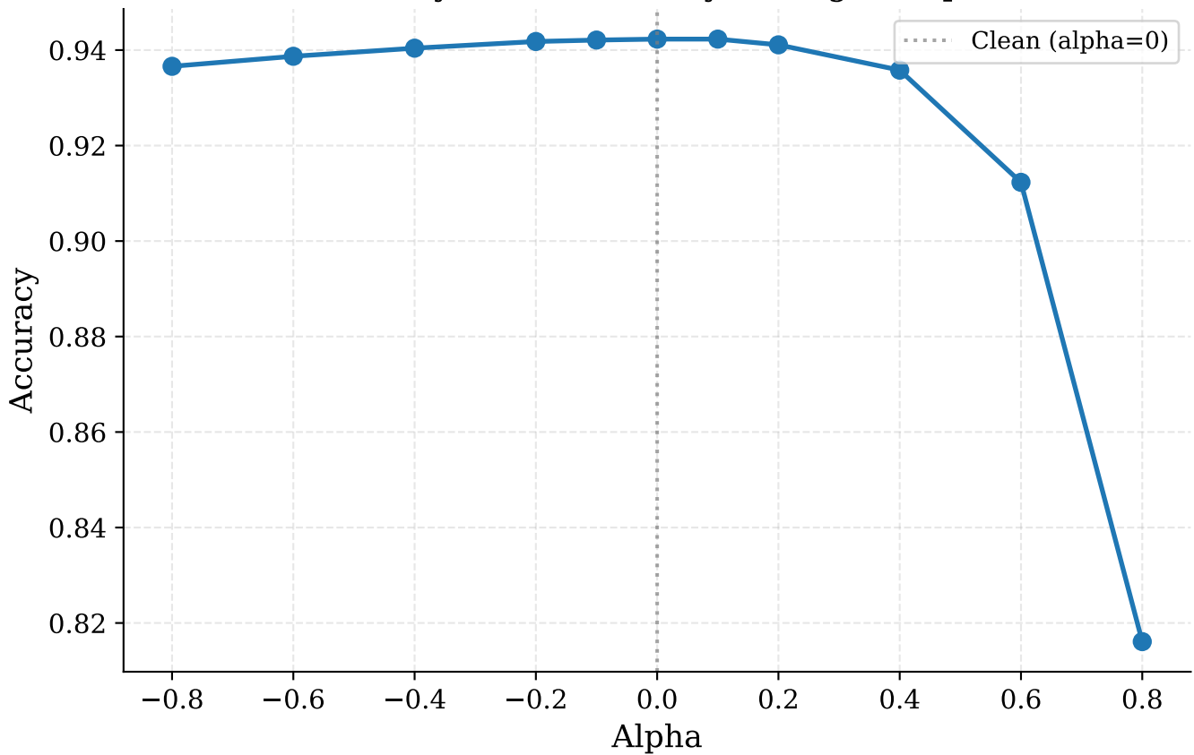
Accuracy vs Nonlinearity Strength (Alpha)
