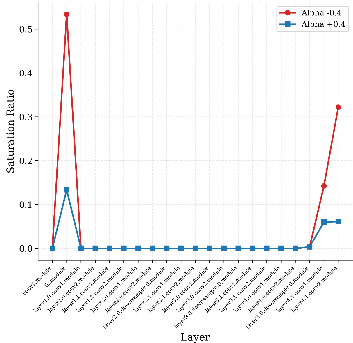
Saturation Ratio Across Layers
