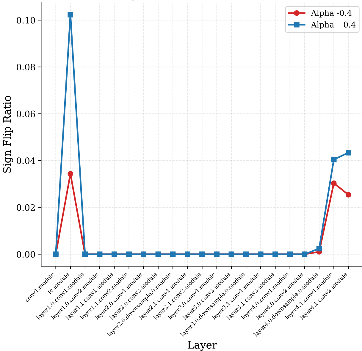
Sign Flip Ratio Across Layers
