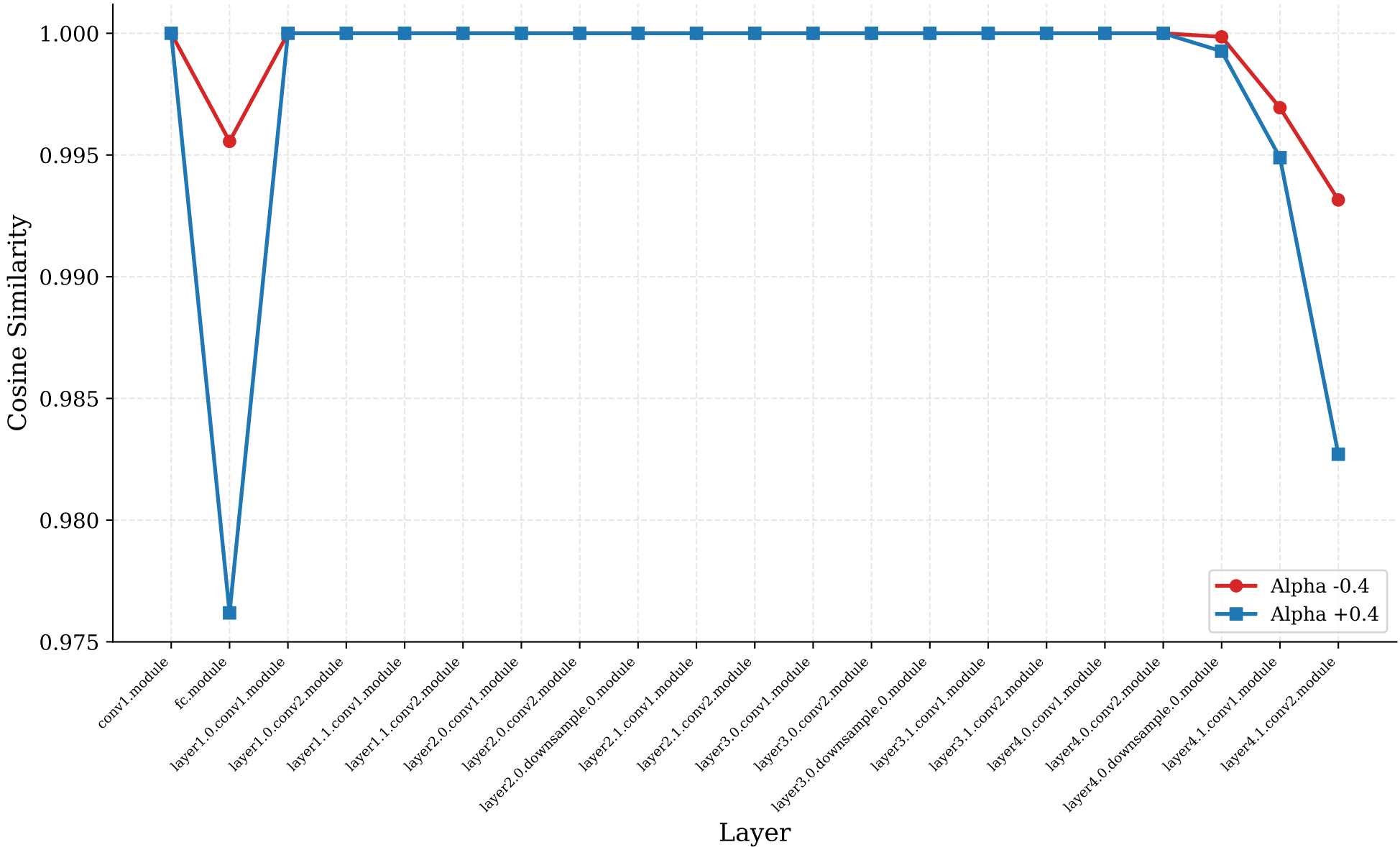
Cosine Similarity Across Layers
