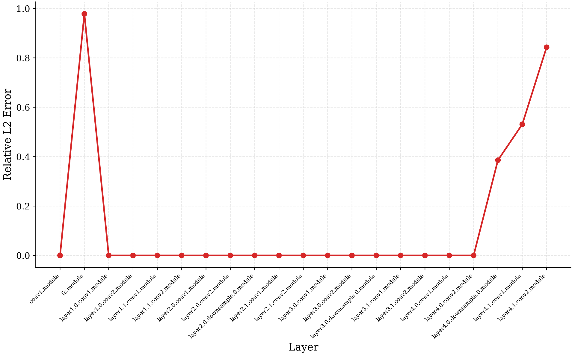
Error Accumulation Across Layers (neg_04)
