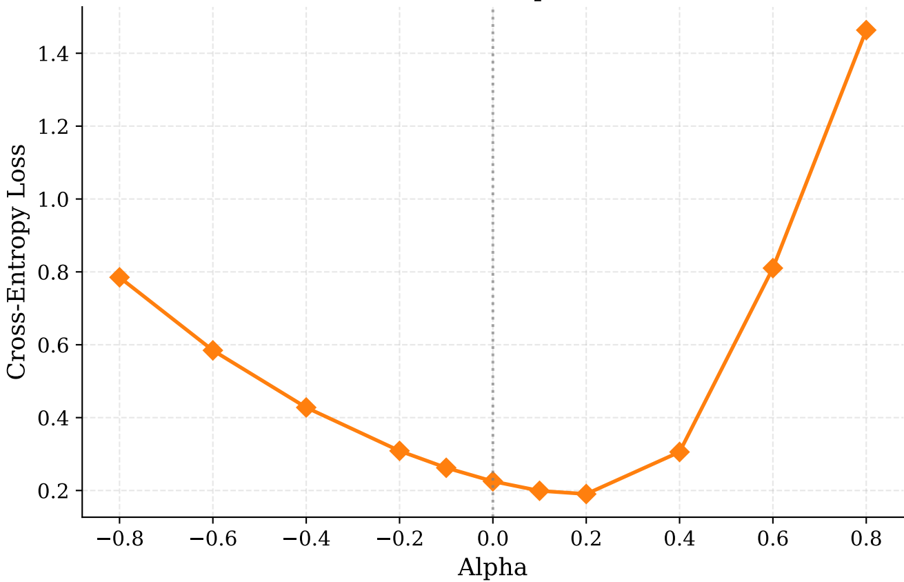
Loss vs Alpha
