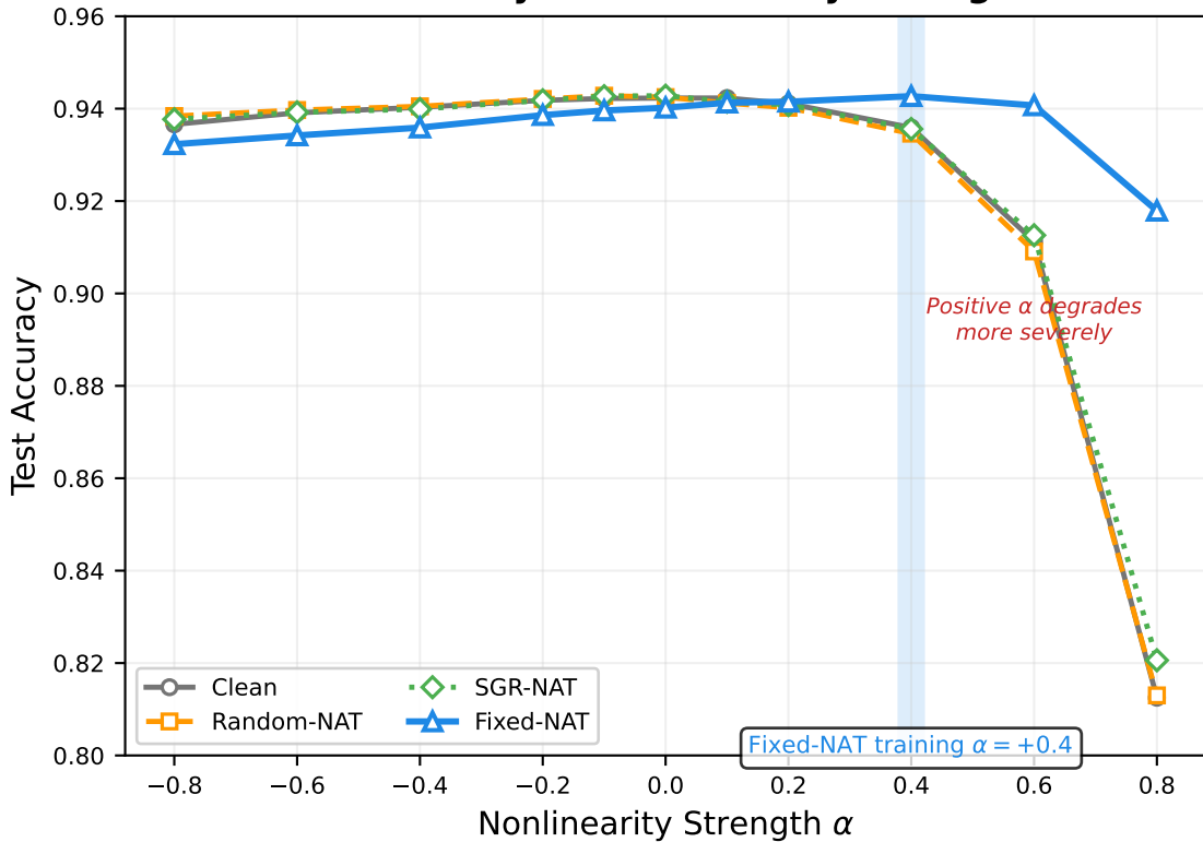
Test Accuracy vs Nonlinearity Strength \alpha
