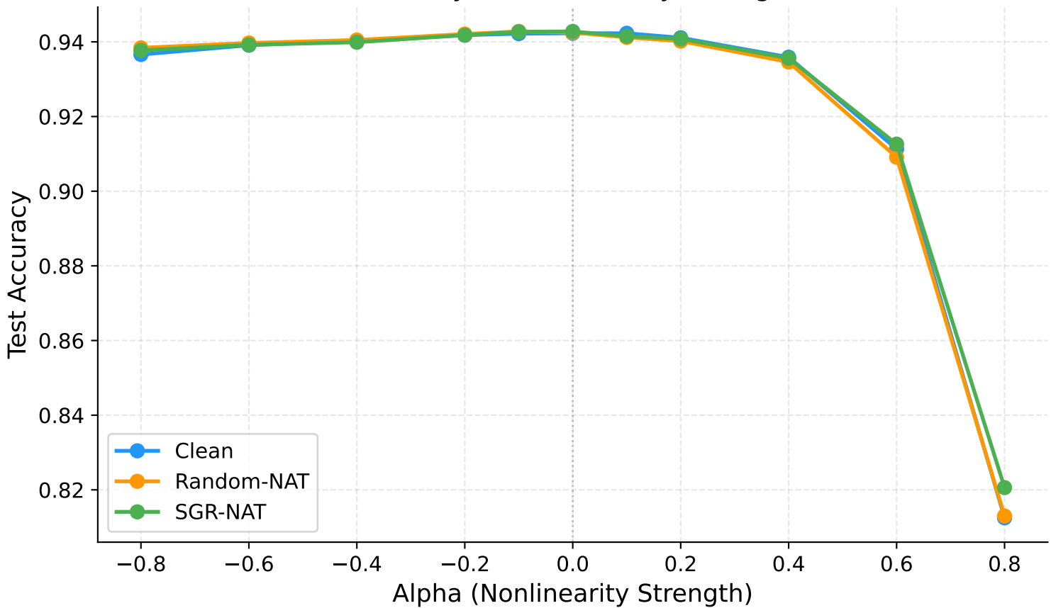
Accuracy vs Nonlinearity Strength
