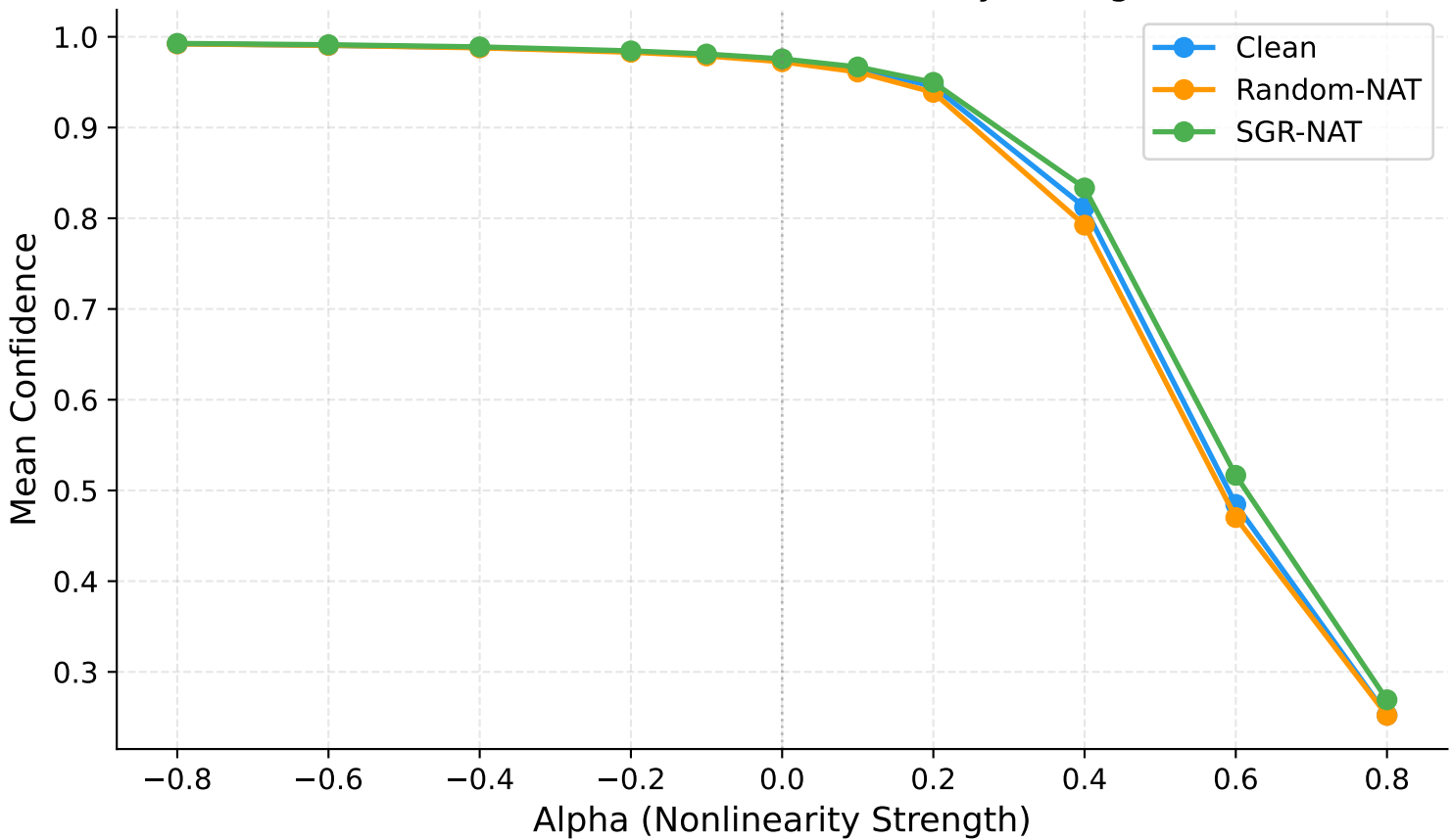
Mean Confidence vs Nonlinearity Strength
