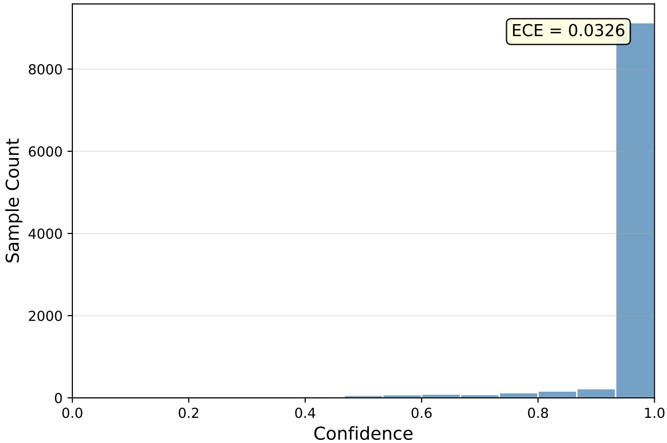
Confidence Histogram: Clean ( \alpha=+0.0 )
