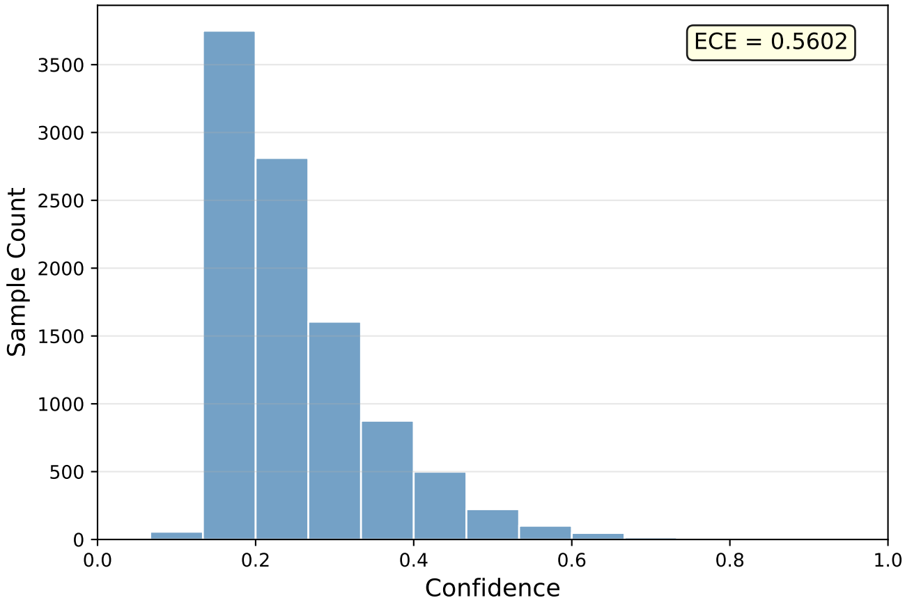
Confidence Histogram: Clean ( \alpha=+0.8 )
