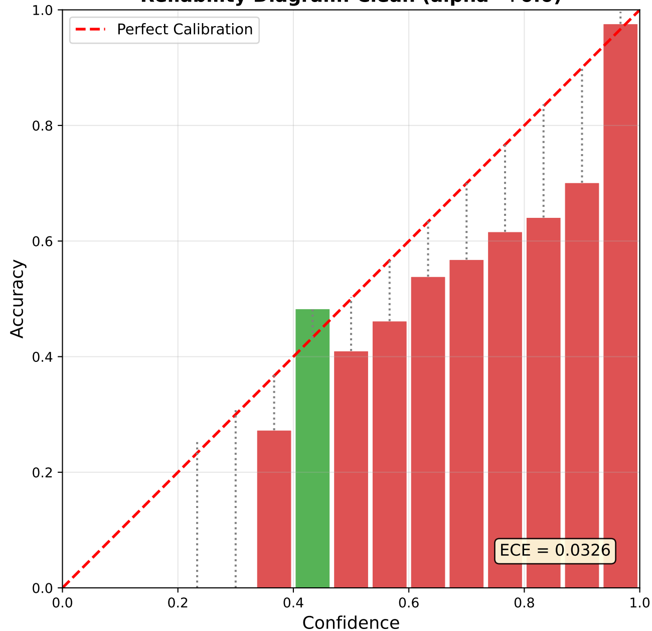
Reliability Diagram: Clean ( \alpha=+0.0 )
