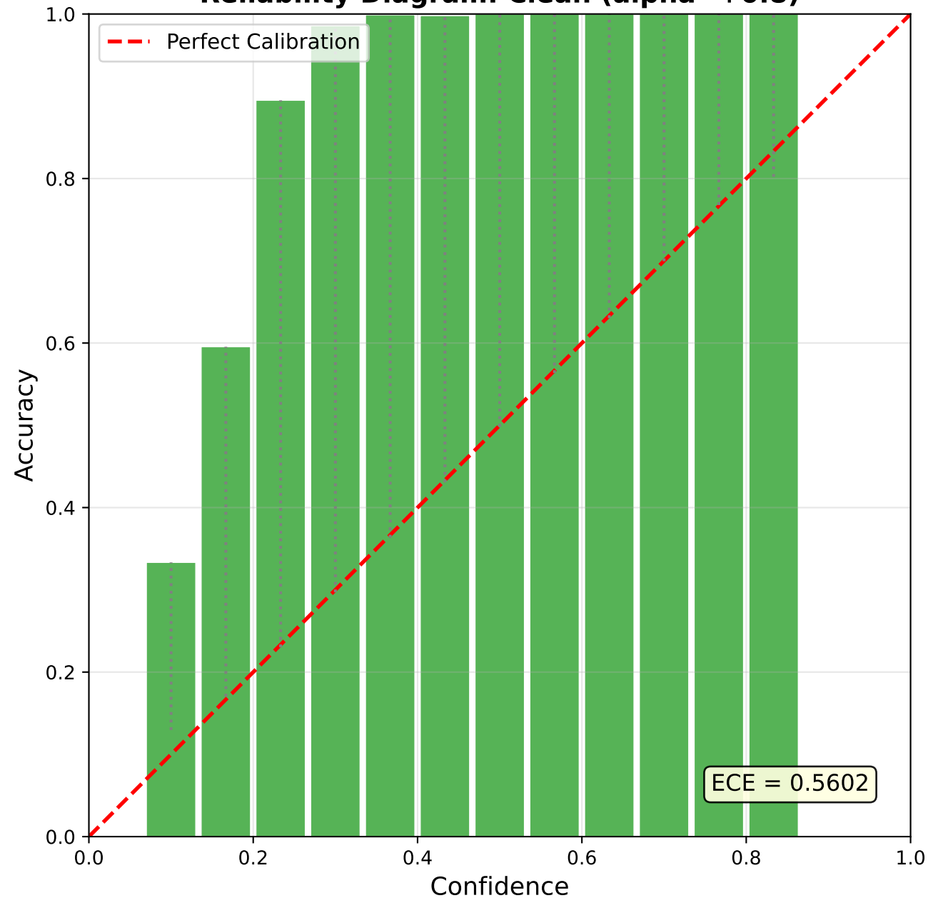
Reliability Diagram: Clean ( \alpha=+0.8 )
