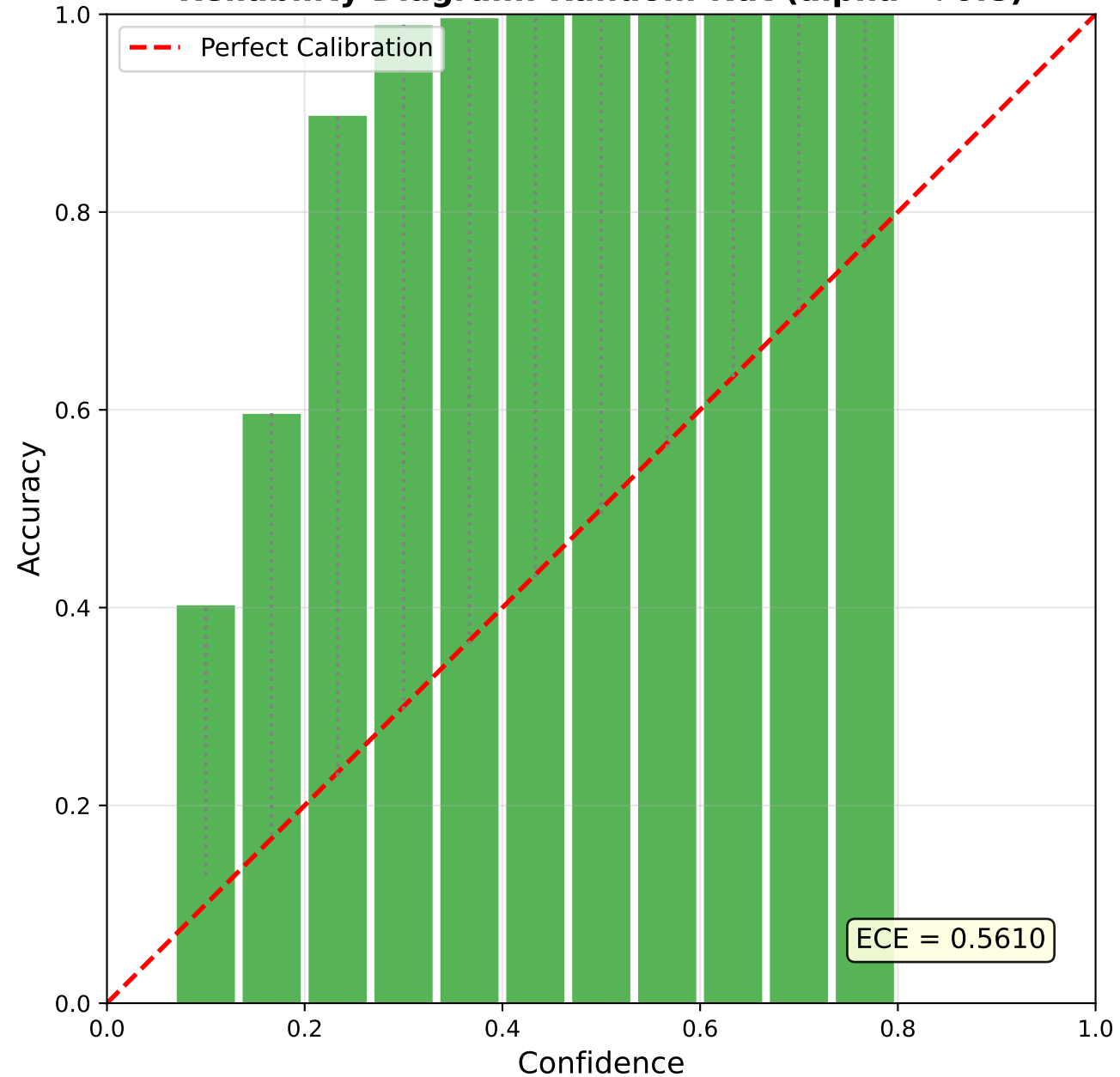
Reliability Diagram: Random-Nat ( \alpha=+0.8 )
