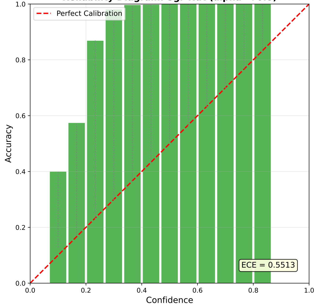
Reliability Diagram: Sgr-Nat ( \alpha=+0.8 )
