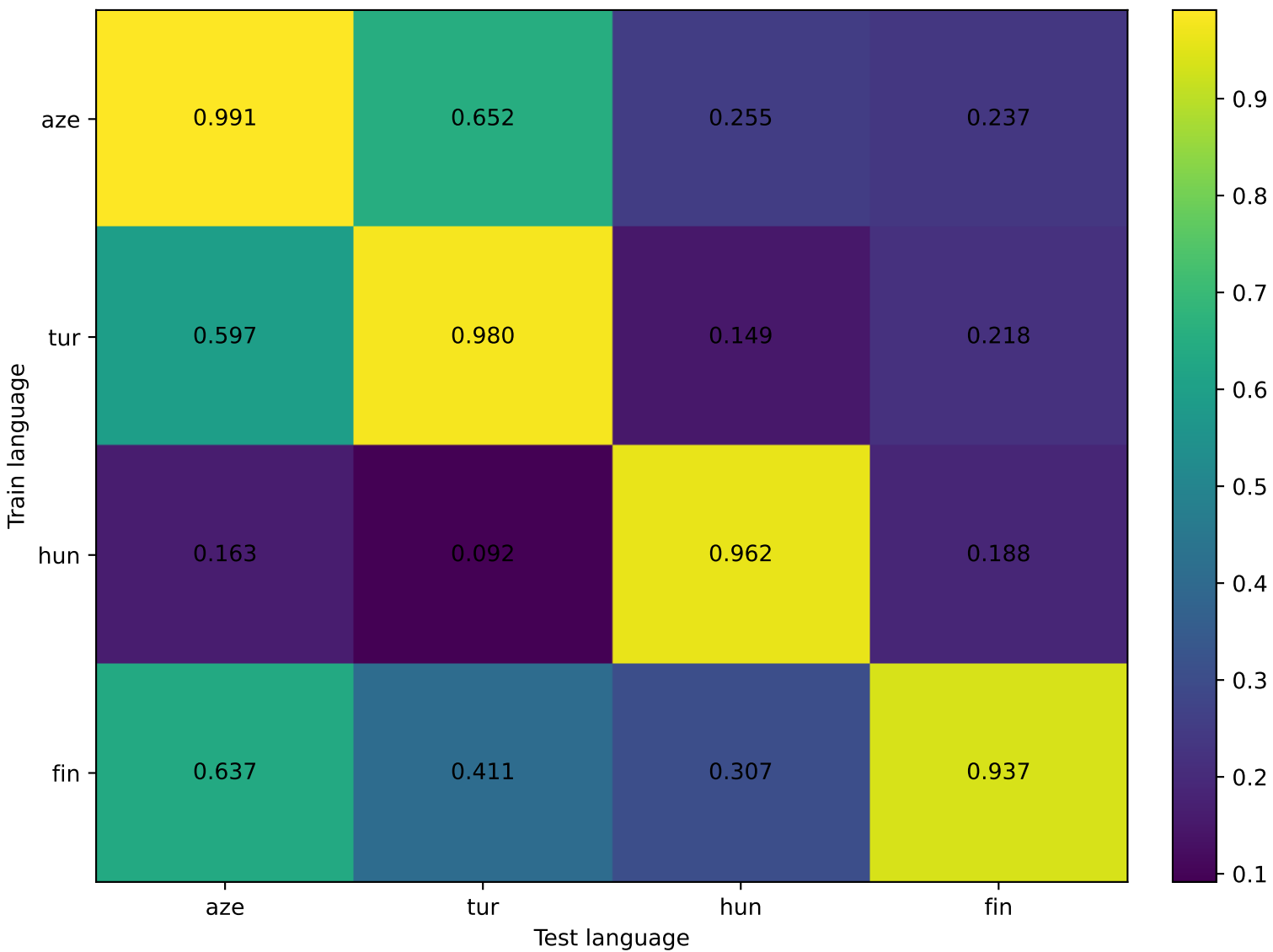
Stem Accuracy Heatmap
