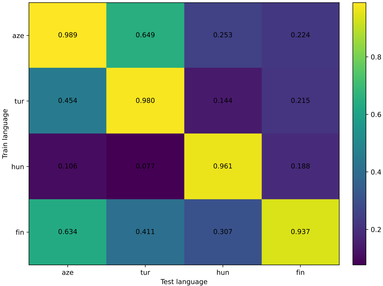
Exact Match Heatmap
