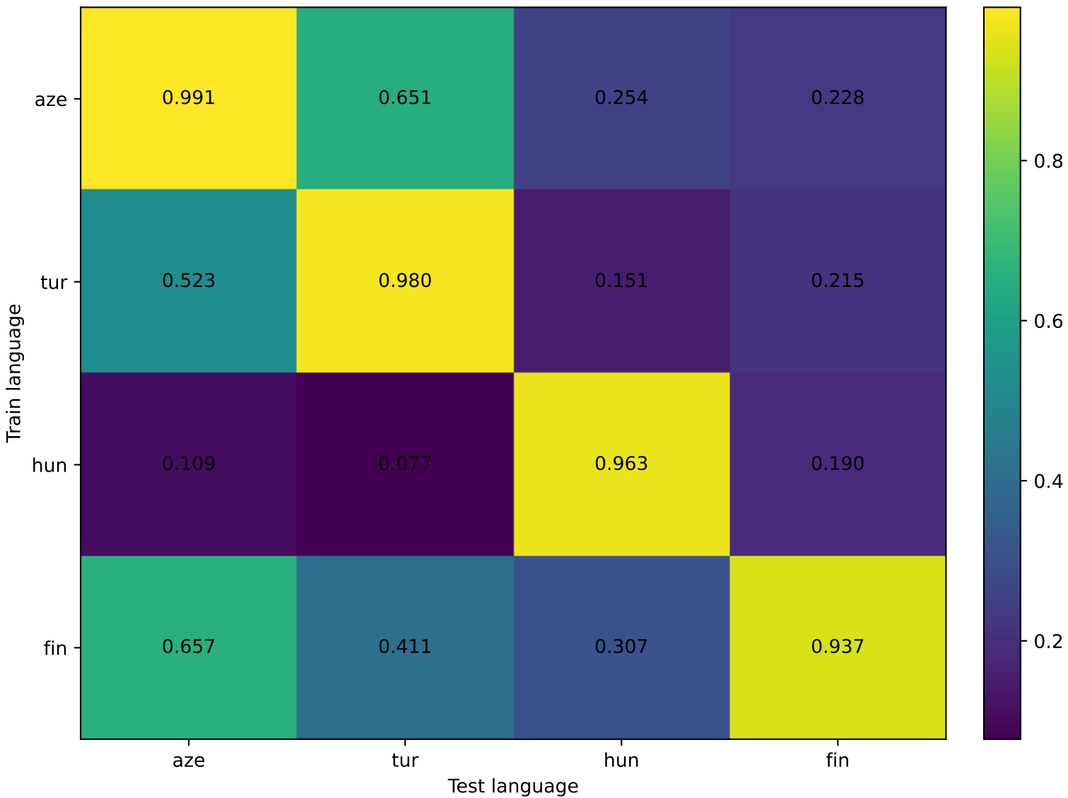
Suffix Accuracy Heatmap
