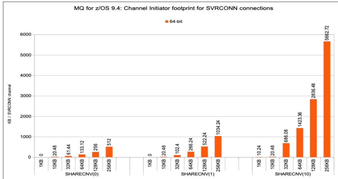
Chart: 64-bit storage usage for MQ 9.4 and later SVRCONN channels
