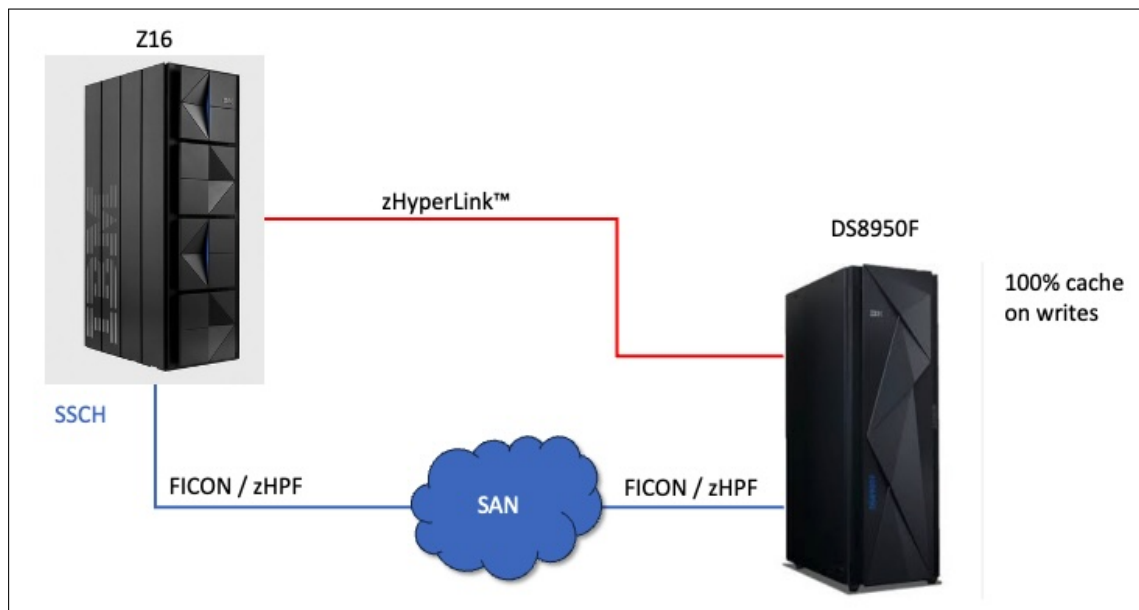
Diagram: Asynchronous and Synchronous I/O paths from mainframe to disk
