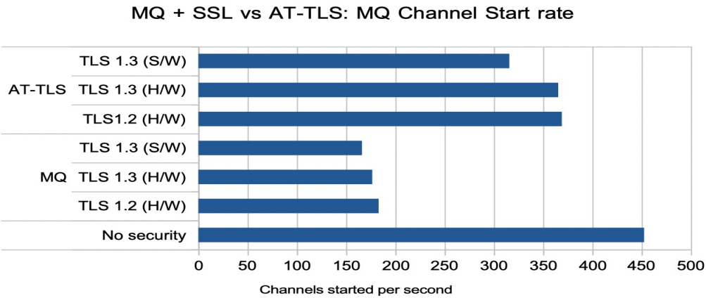
Chart: Start channel rate
