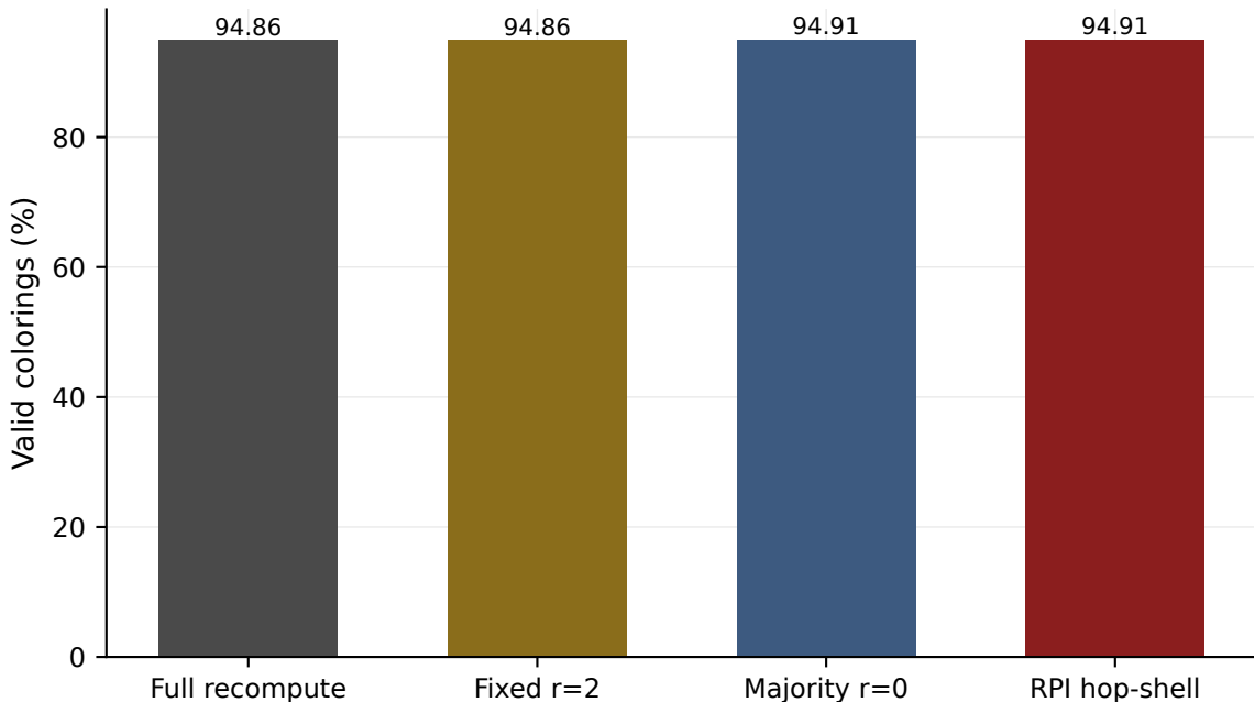
Validity is shared with full recompute (holdout, 2,025 edits)
