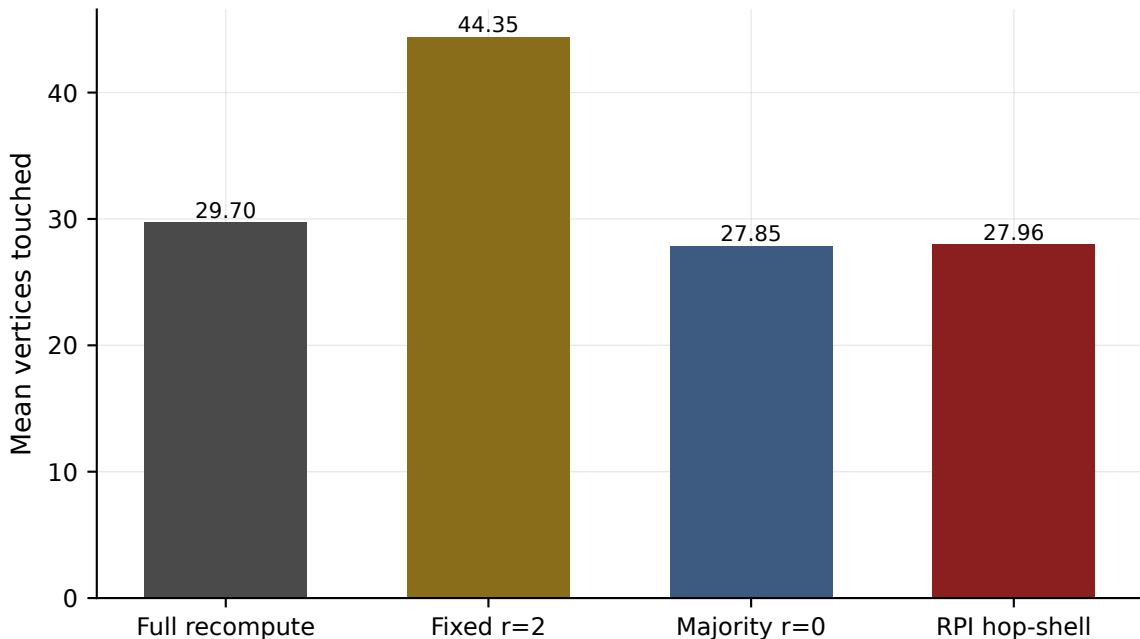
RPI touches fewer vertices than fixed r=2 (−37% mean)
