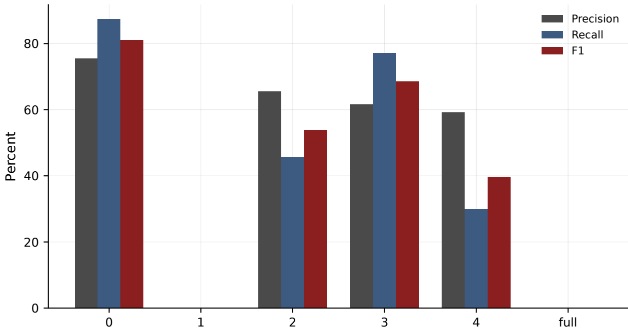
Per-class precision / recall / F1 (class 1 and full are never predicted)
