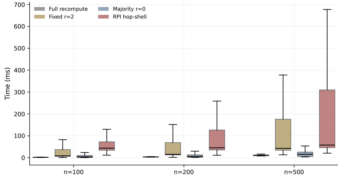
Time by system and n (medians; outliers hidden)
