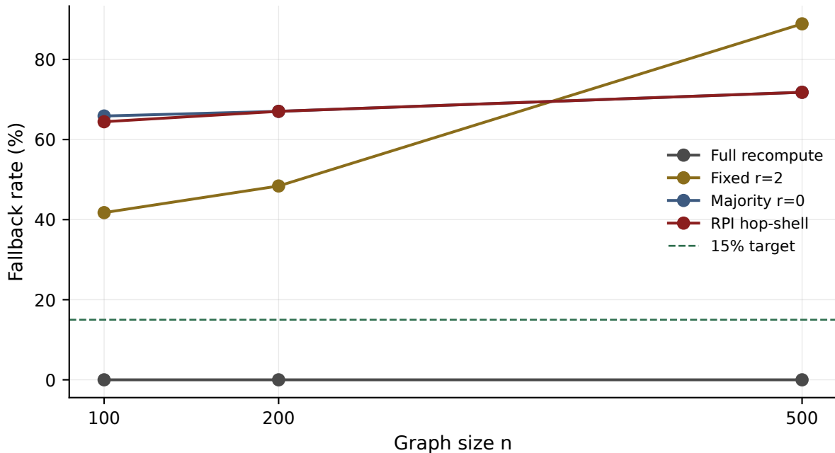
Holdout fallback vs n (fixed r=2 collapses at n=500)
